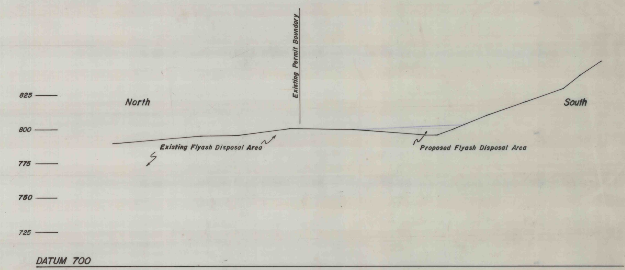
CROSS-SECTION H-H Looking East
