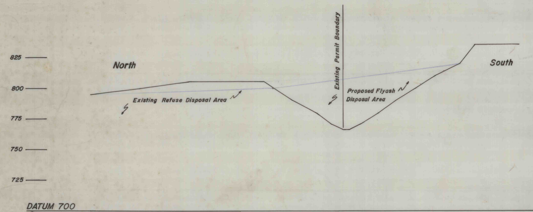
CROSS-SECTION F-F Looking East
