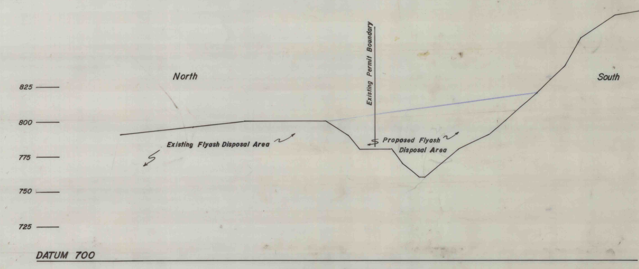
CROSS-SECTION G-G Looking East
