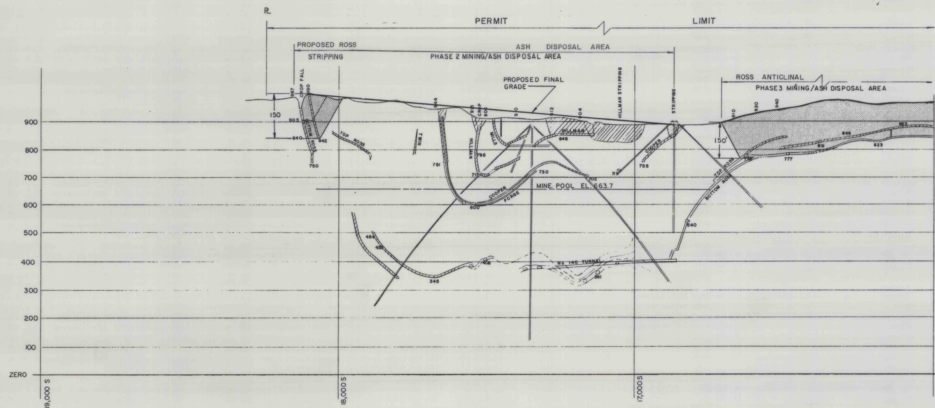
SECTION LINE 12 LOOKING WEST
