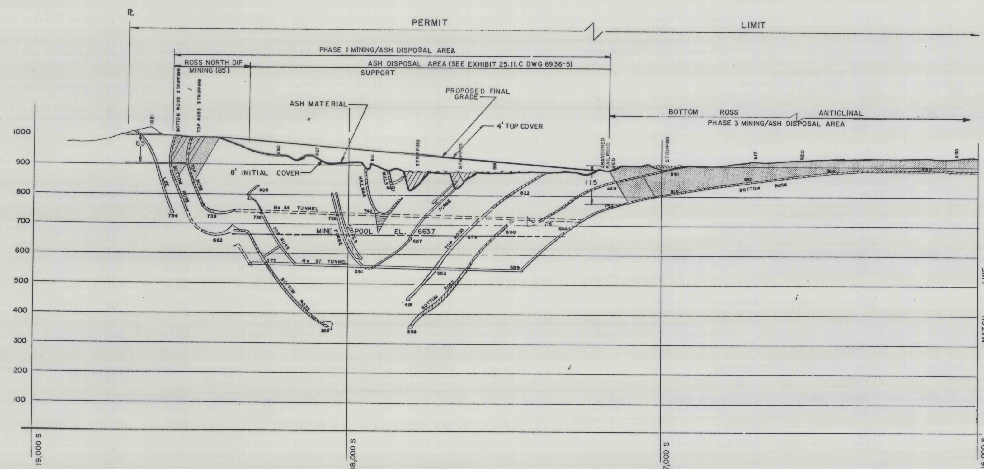
SECTION LINE 8 1/2 LOOKING WEST
