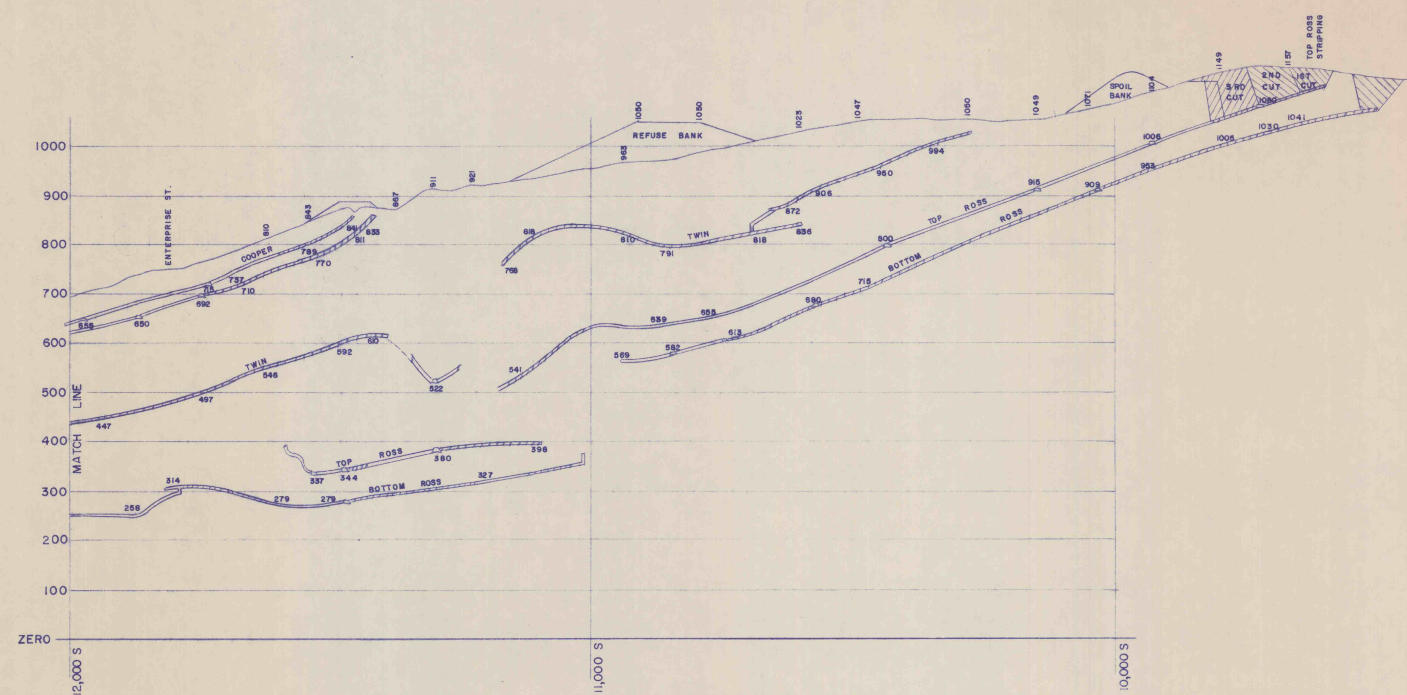
SECTION LINE 14+250
