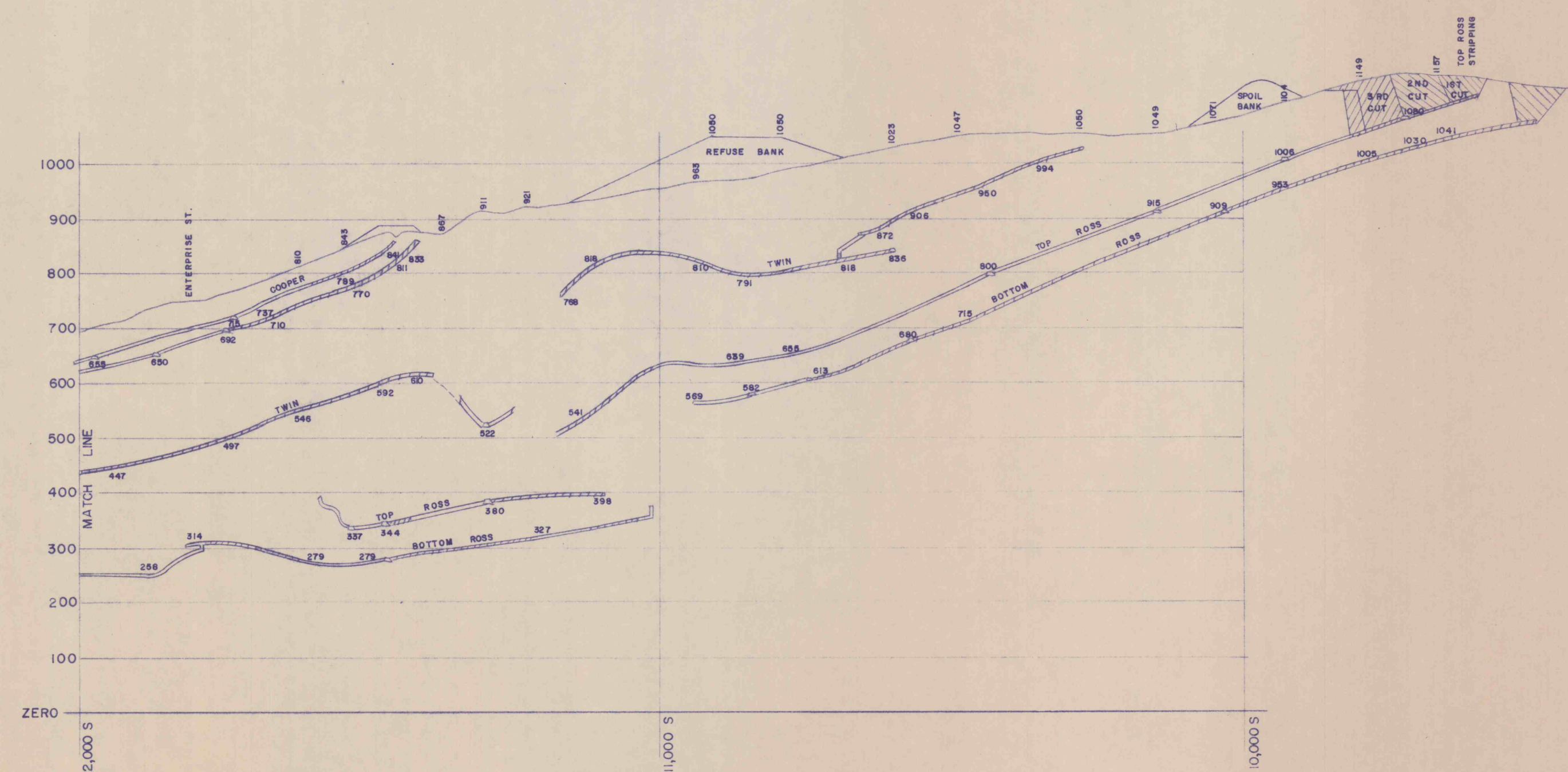
SECTION LINE 14+250
