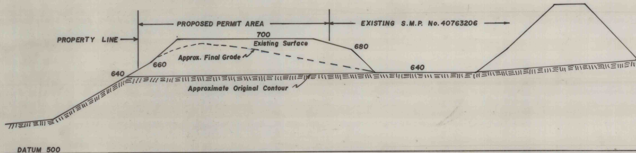
SECTION B-B LOOKING WEST
