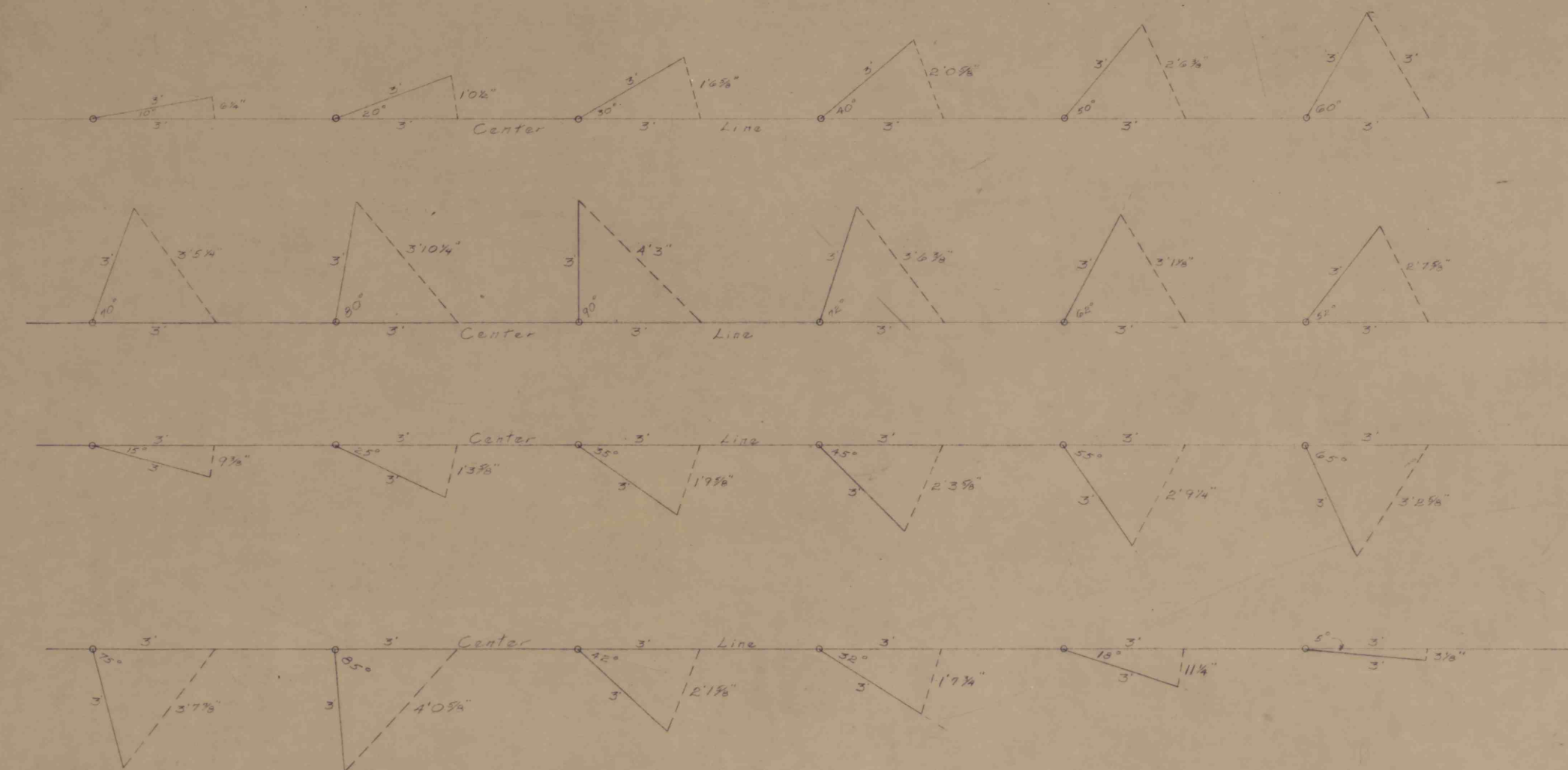
METHODS OF TURNING ANGLES FROM THE CENTER LINE
