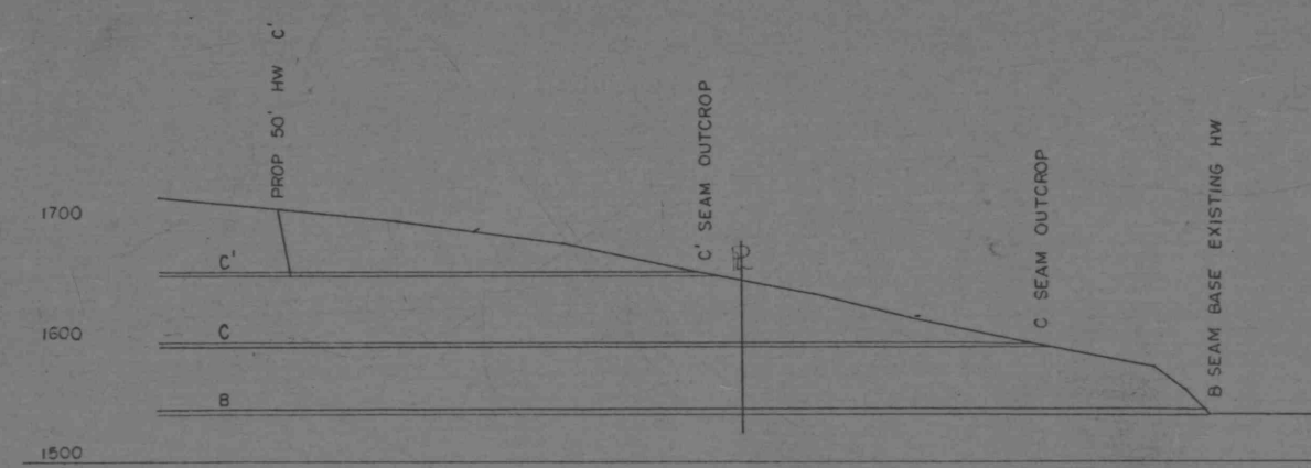
SECTION 48-48'
