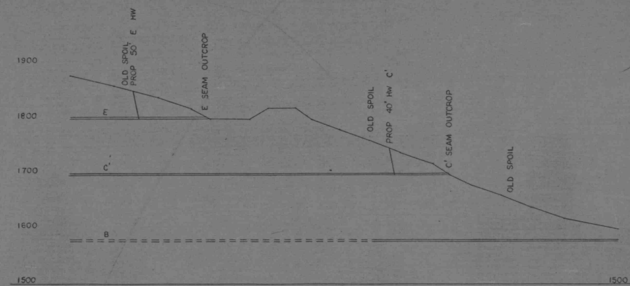
SECTION 46-46'
