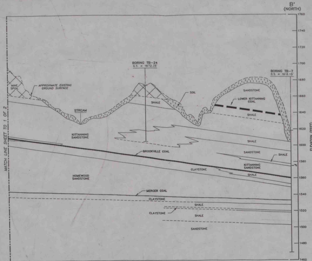
GEOLOGIC CROSS SECTION B-B' (LOOKING WEST) 10X VERTICAL EXAGGERATION
