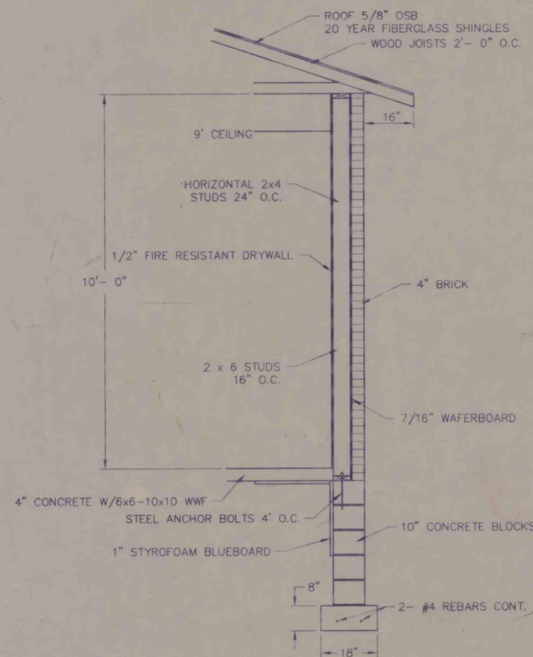
TYPICAL WALL SECTION BRICK SCALE: 1/2" = 1' - 0"
