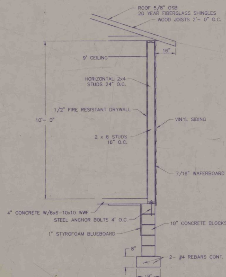
TYPICAL WALL SECTION SIDING SCALE: 1/2" = 1' - 0"
