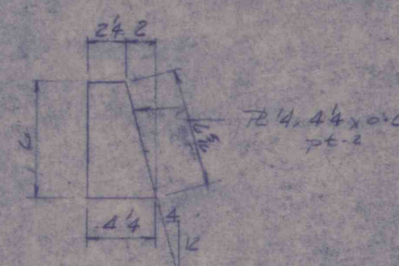
30° ROOF
