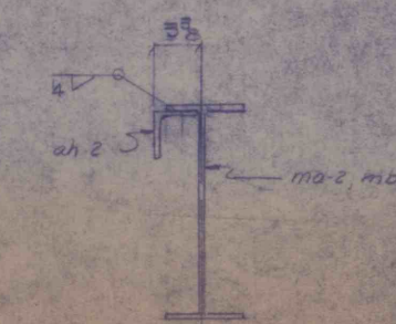
HOOP ANGLE DETAIL
