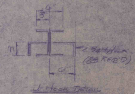
J-Hook Detail
