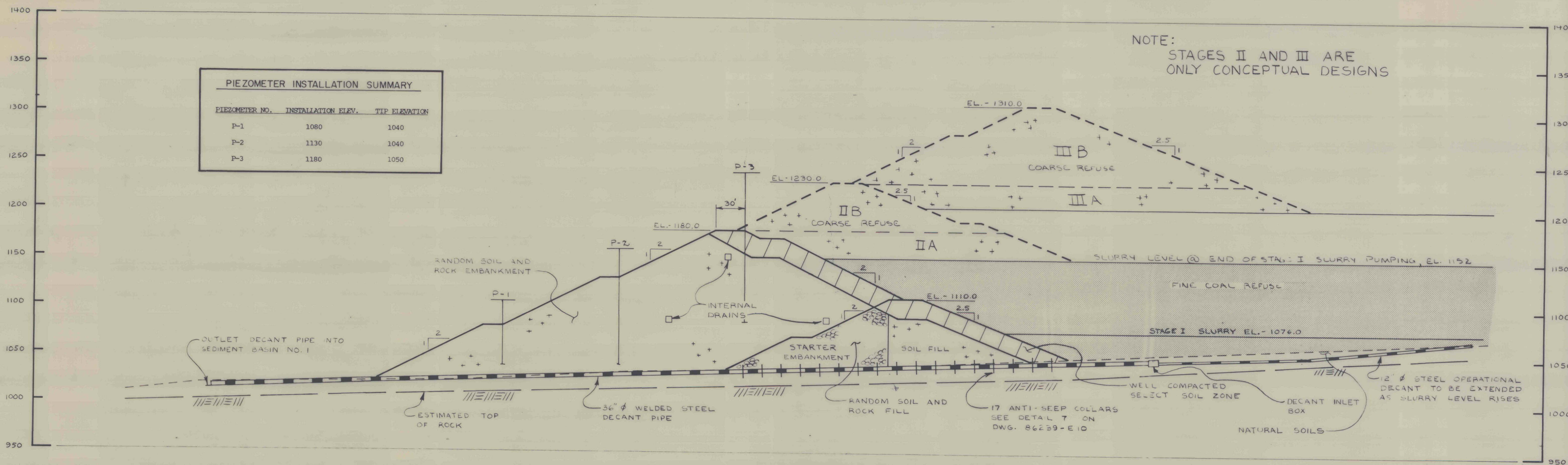
GENERALIZED SECTION THROUGH THE IMPOUNDMENT
