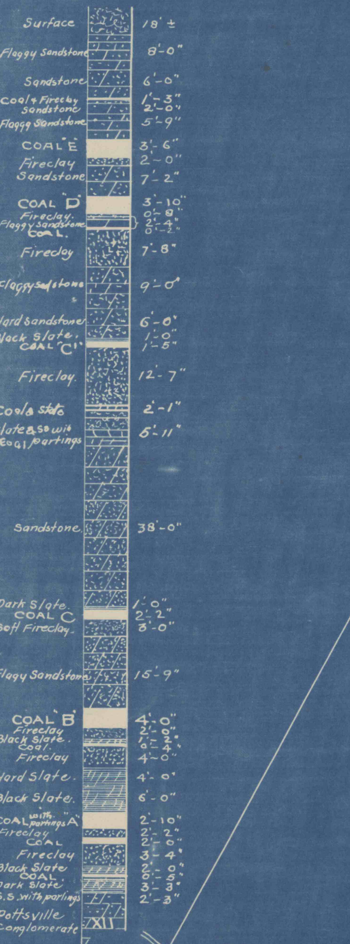
COLUMNAR SECTION - BORE HOLE B.
