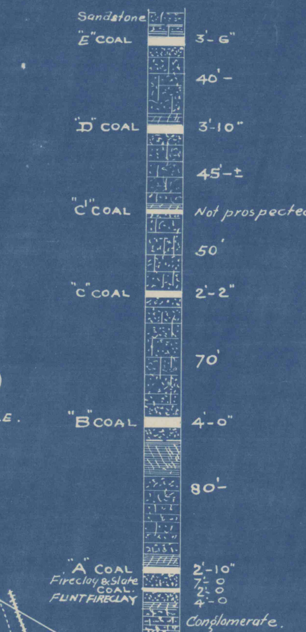
COLUMNAR SECTION AT A
