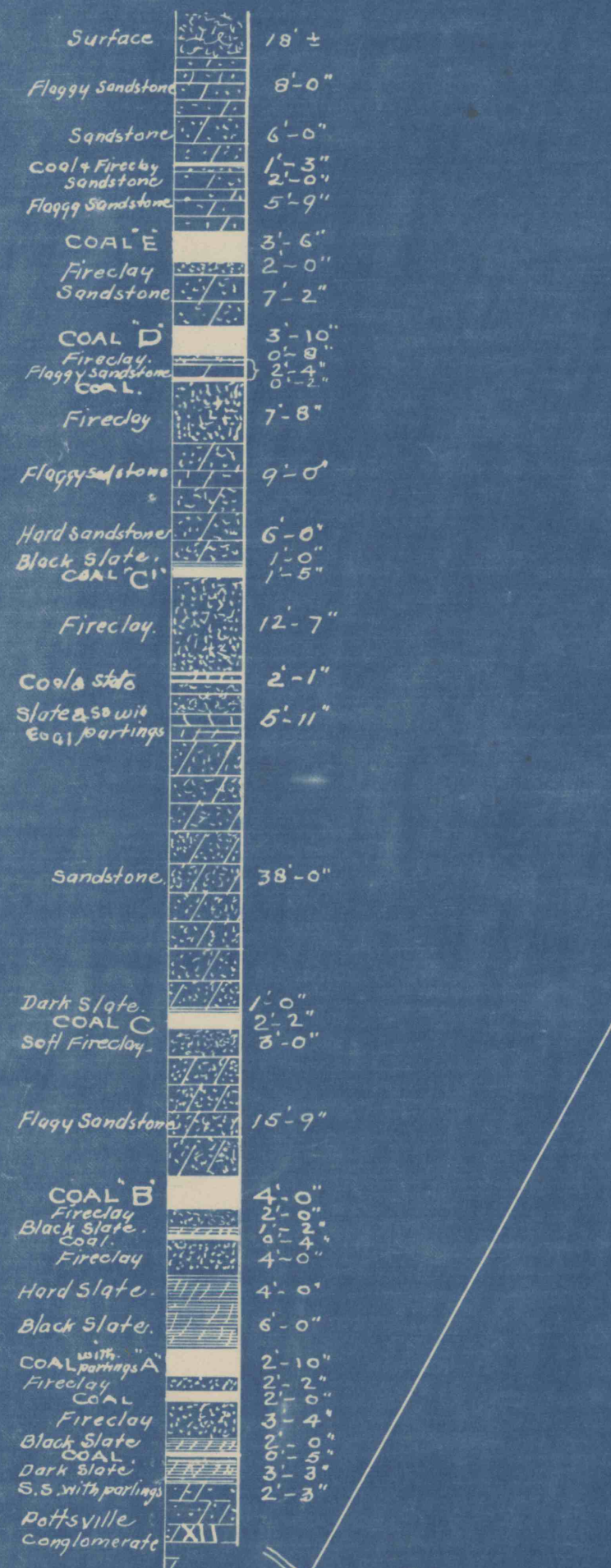
COLUMNAR SECTION - BORE HOLE B.
