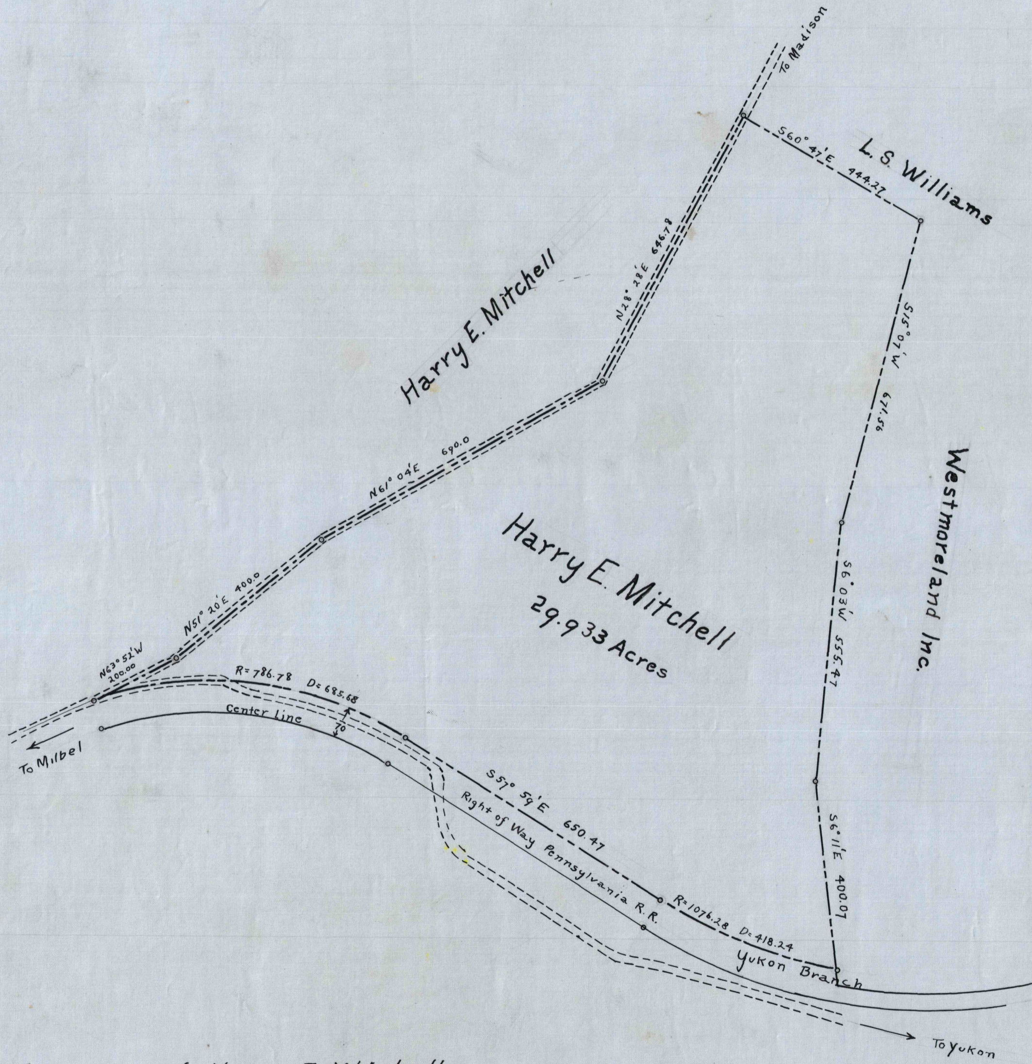
Plot of Portion of Harry E Mitchell Tract of Land in Sewickley Township Westmoreland County Pa. Scale 200ft = 1 in. Nov. 23. 1929
