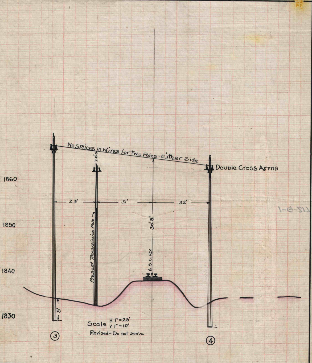
SOMERSET COAL CO. PLAN AND PROFILE SHOWING PROPOSED 2300 VOLT TRANSMISSION LINE CROSSING THE SOMERSET COAL RY. NEAR GRAY, PA. JENNER TWP. SOMERSET CO. PA. 8-1-19 Engr. Dept. Pa. Div.
