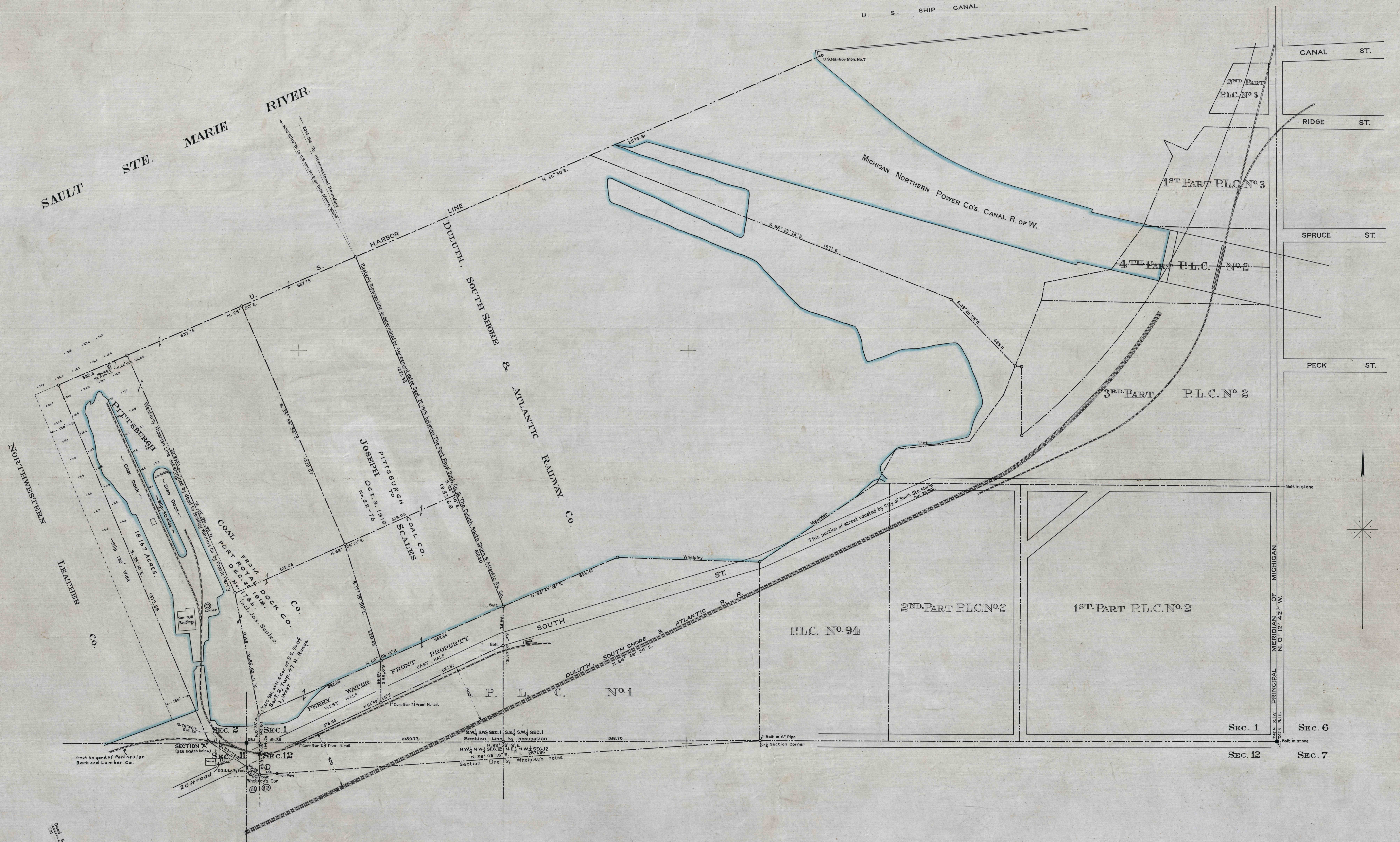
PLAN OF PITTSBURGH COAL CO'S ALGONQUIN DOCK PROPERTY SITUATE AT SAULT STE. MARIE, CHIPPEWA CO., MICH. Scale 1" = 200' Oct. 31, 1918.
