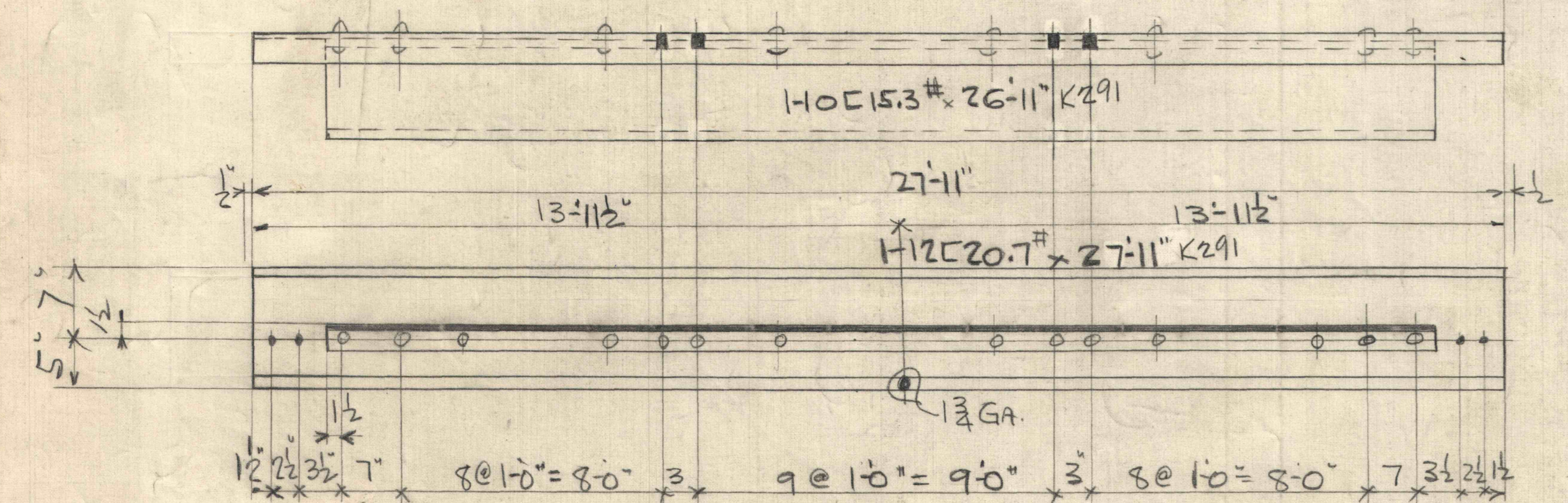
5 - PURLIN - P9
