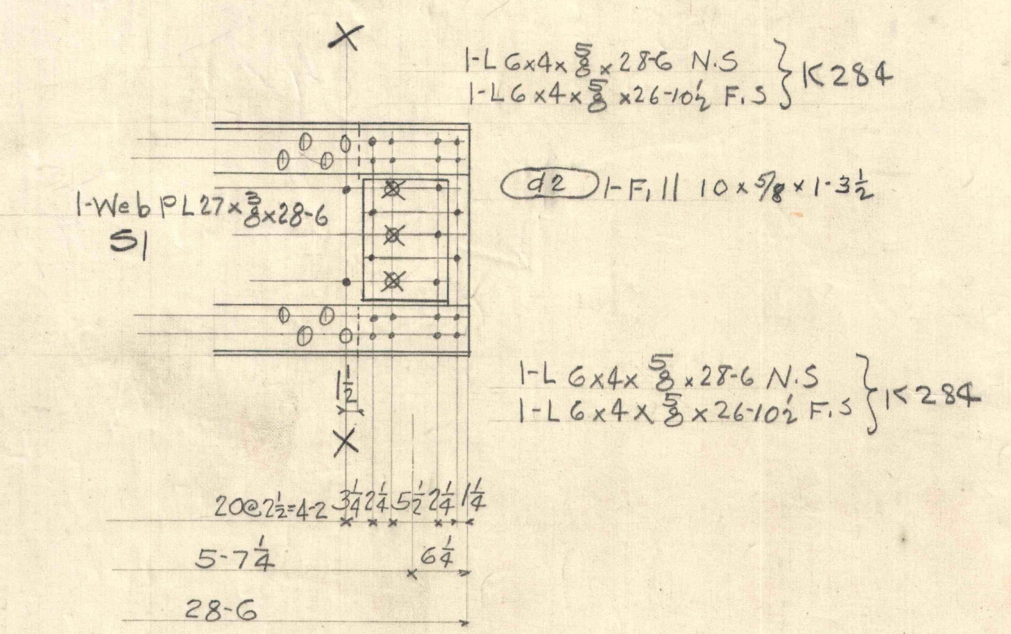
One Girder G8 Balance of Details same as G7
