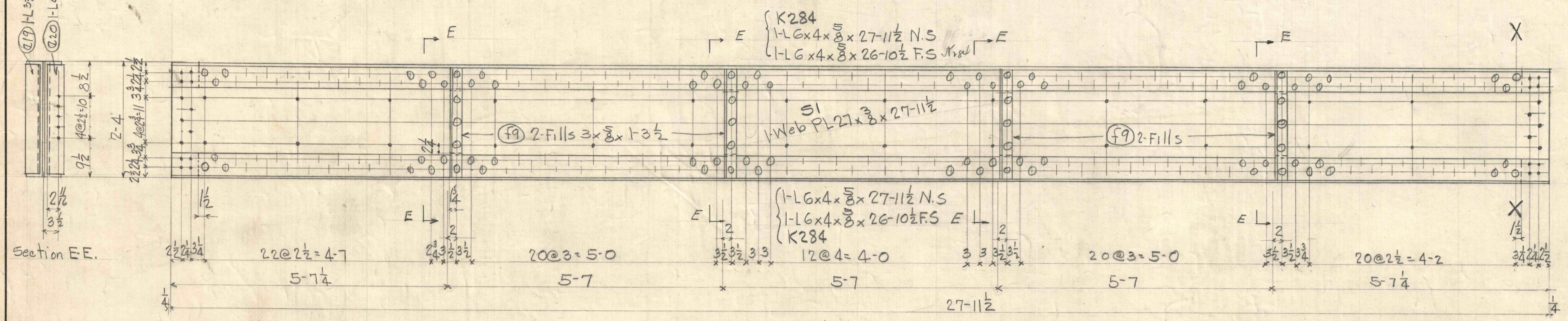
2-Girders G7
