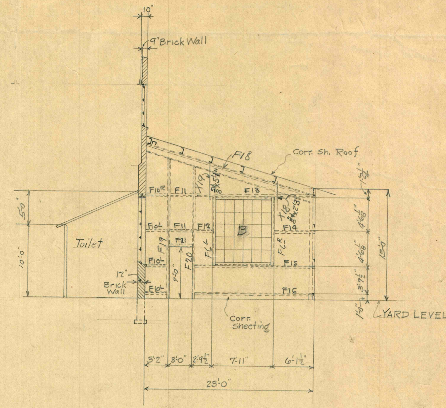
SECTION F-F
