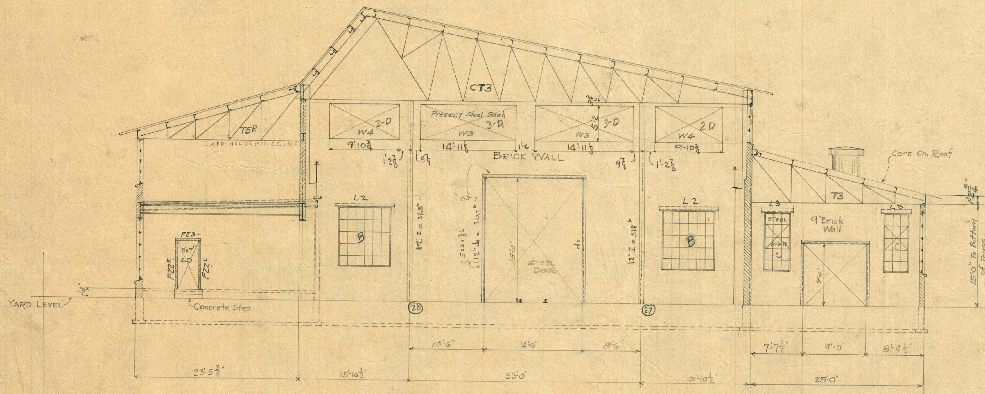
SECTION of SOUTH ELEVATION E-E
