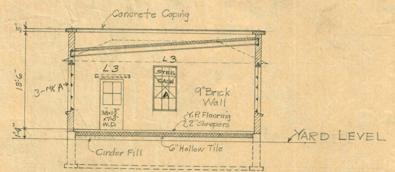
SECTION H-H
