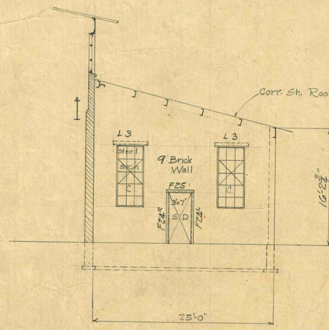
SECTION - G-G
