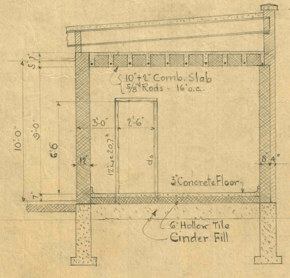
SECTION 3-3
