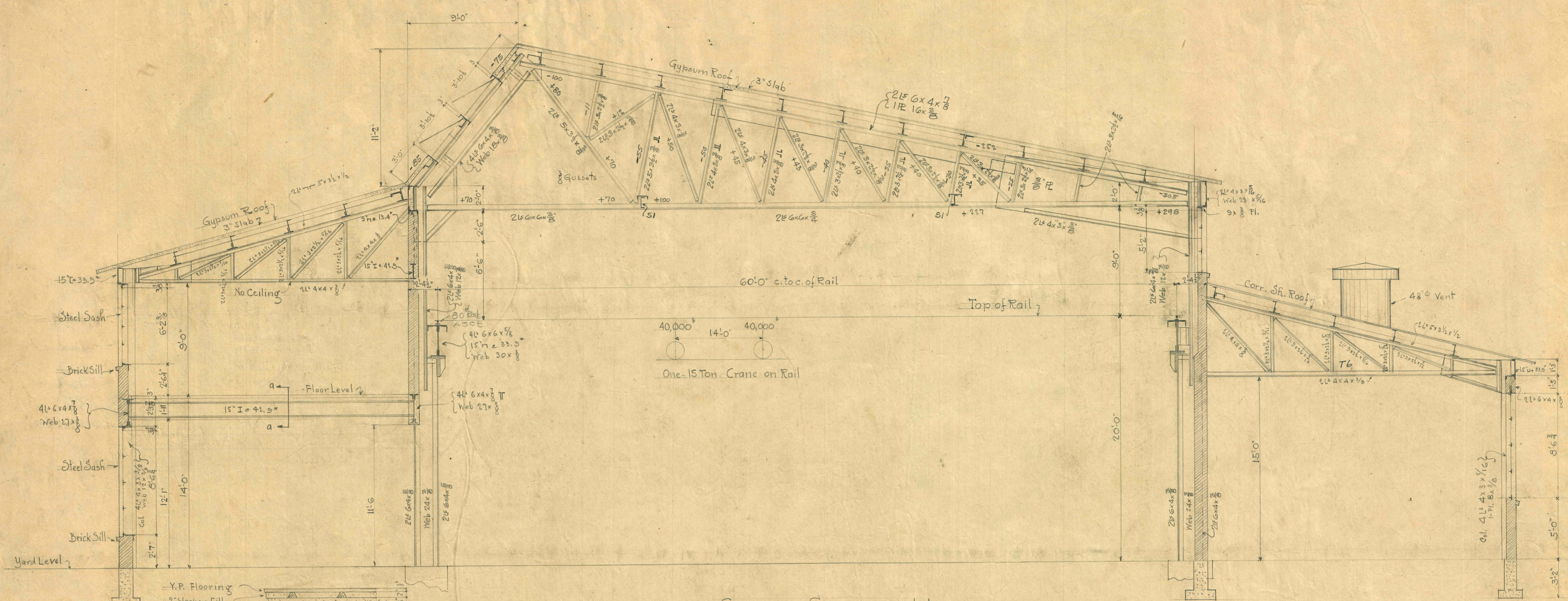
CROSS SECTION 1-1
