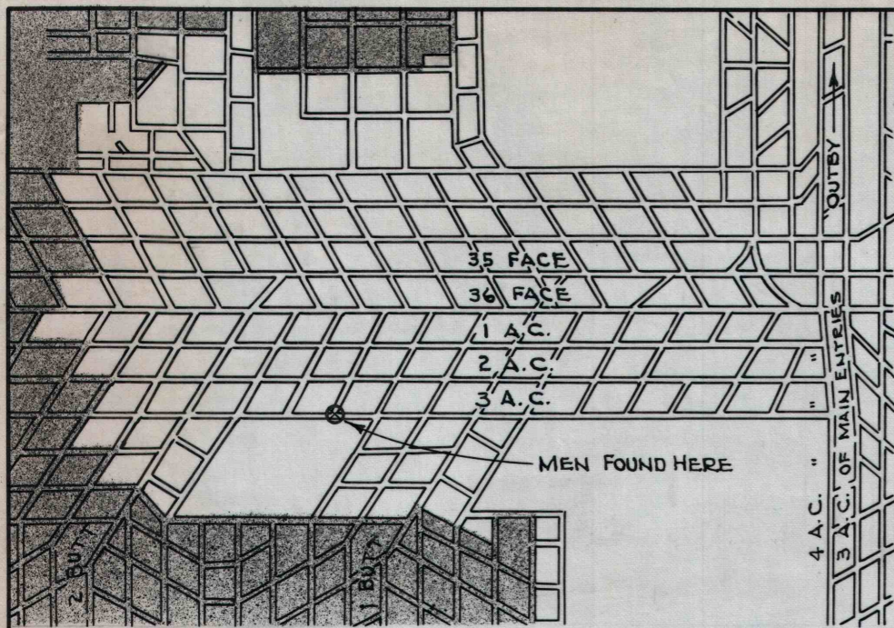
GENERAL PLAN SCALE: 1" = 400'
