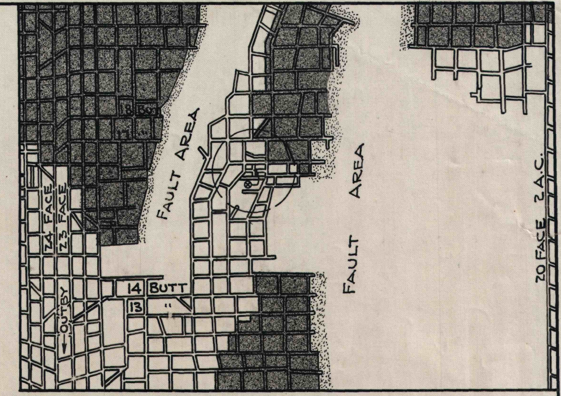
GENERAL PLAN SCALE 1"=400'
