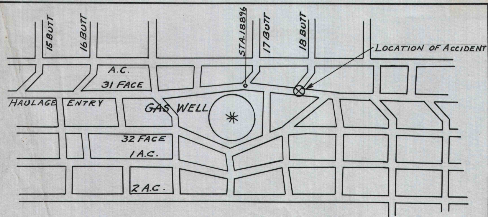
GENERAL PLAN SCALE 1"=100'
