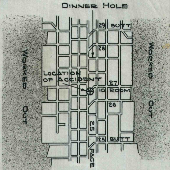
GENERAL PLAN SCALE 1" = 400'
