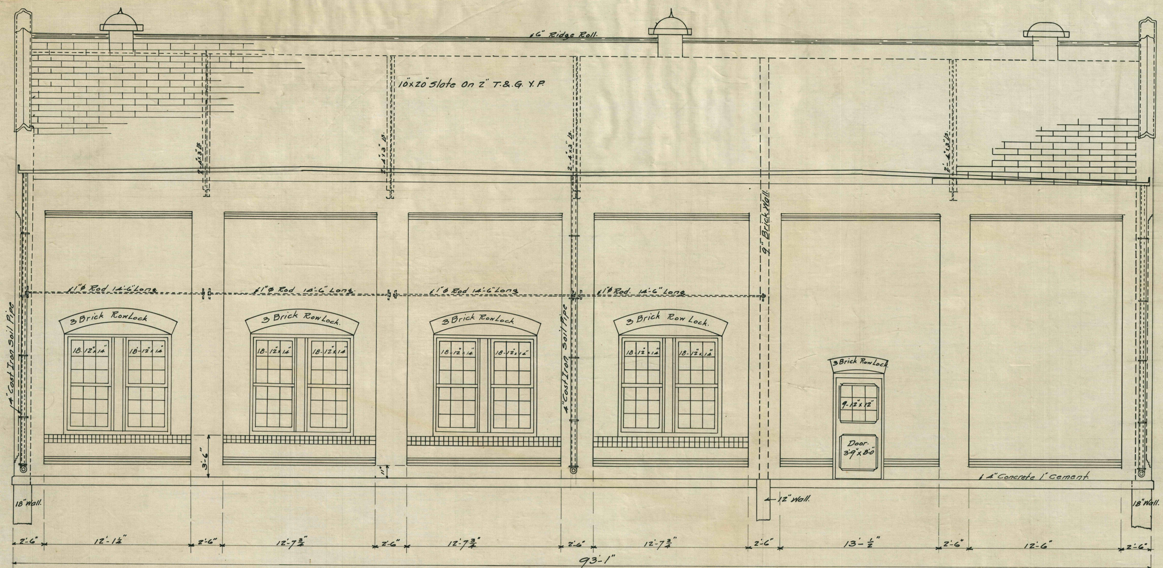
WESTERN ELEVATION.
