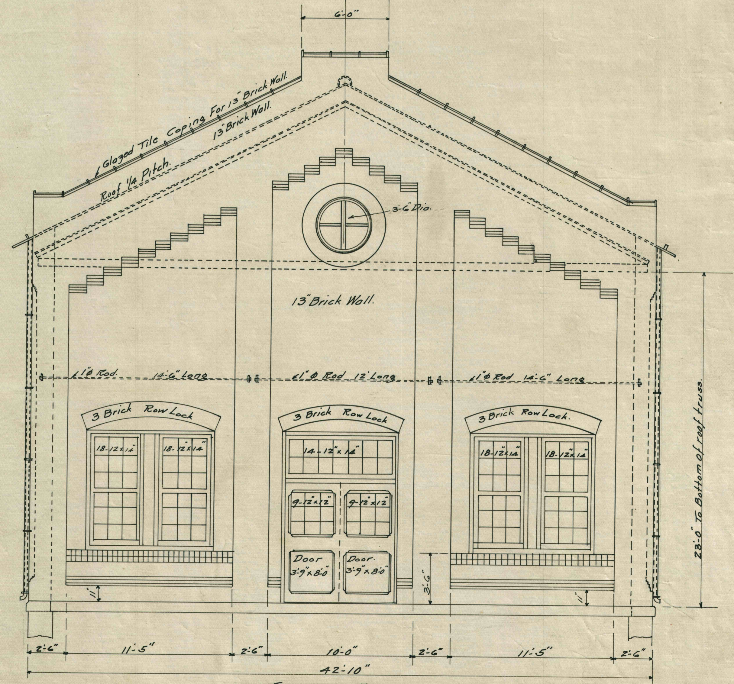
SOUTHERN ELEVATION.
