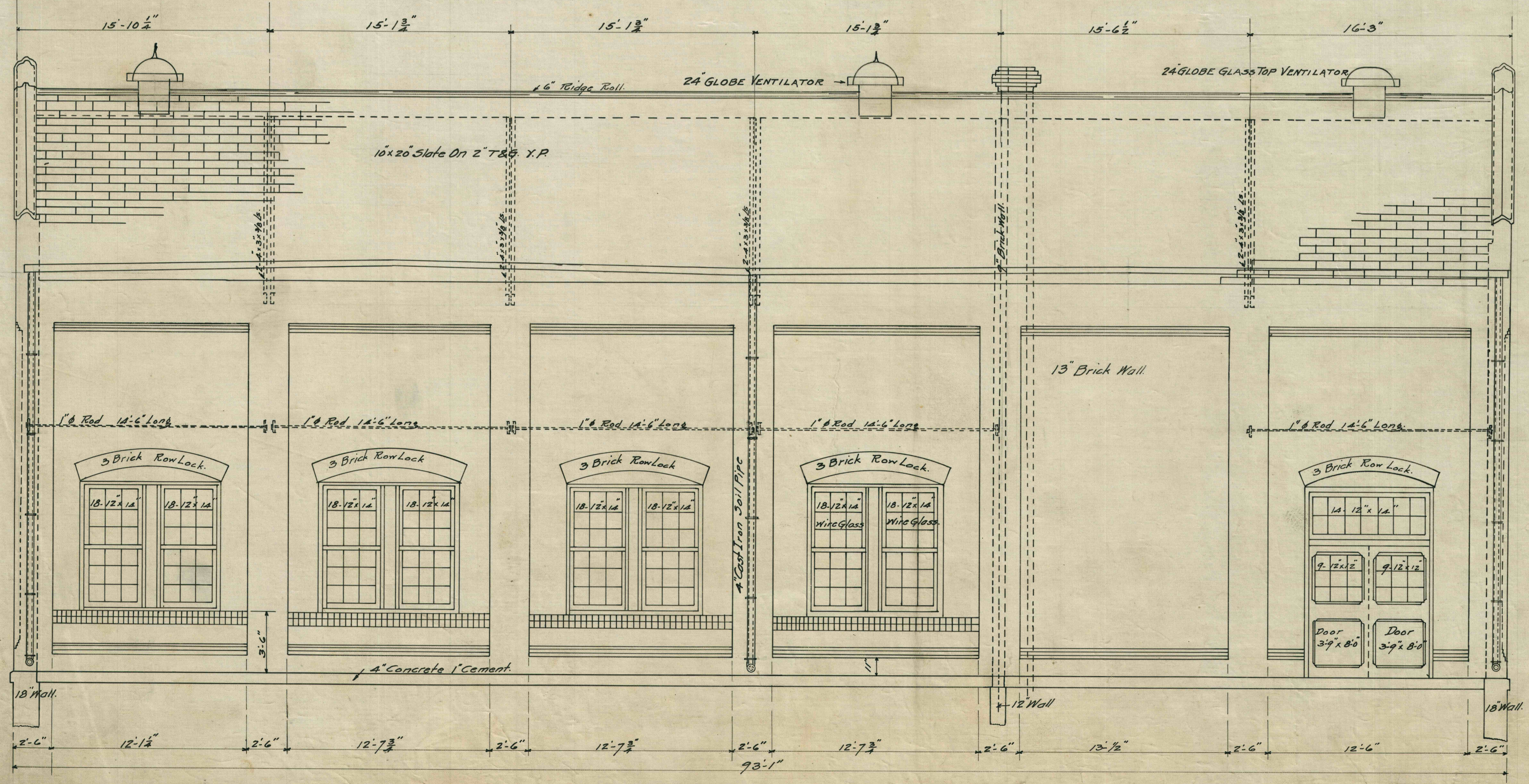
EASTERN ELEVATION.
