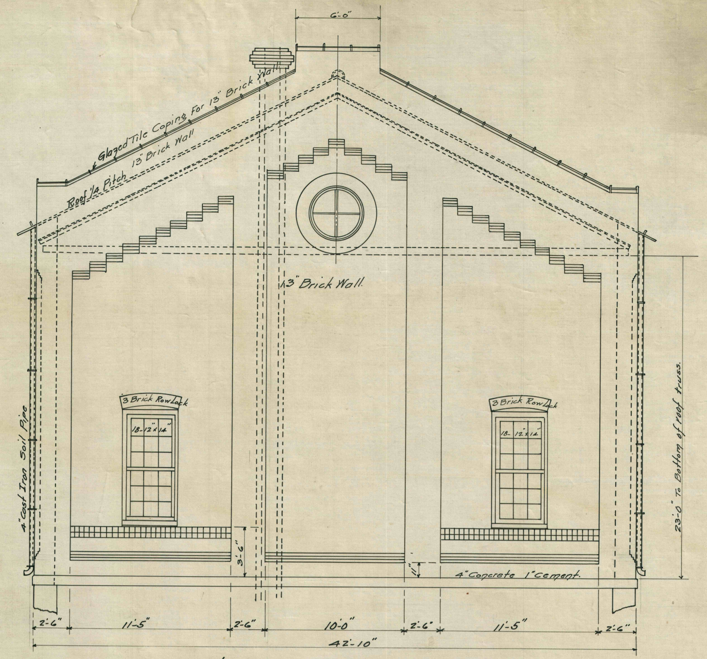
NORTHERN ELEVATION.
