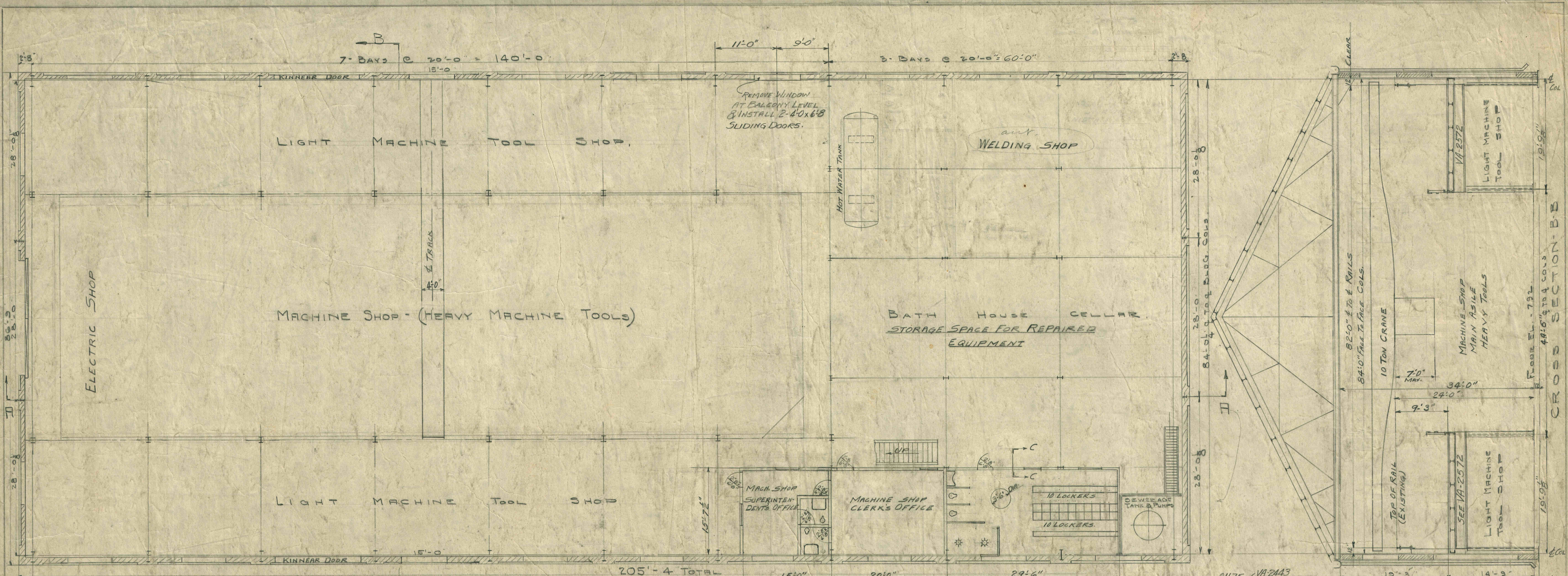
PLAN OF MACHINE SHOP - 1ST OR MAIN FLOOR SCALE - 1/8" = 1'-0"
