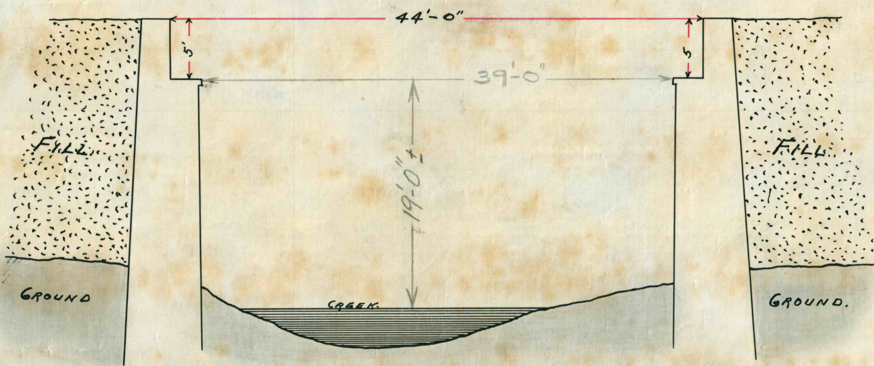
Section on Line A-B.
