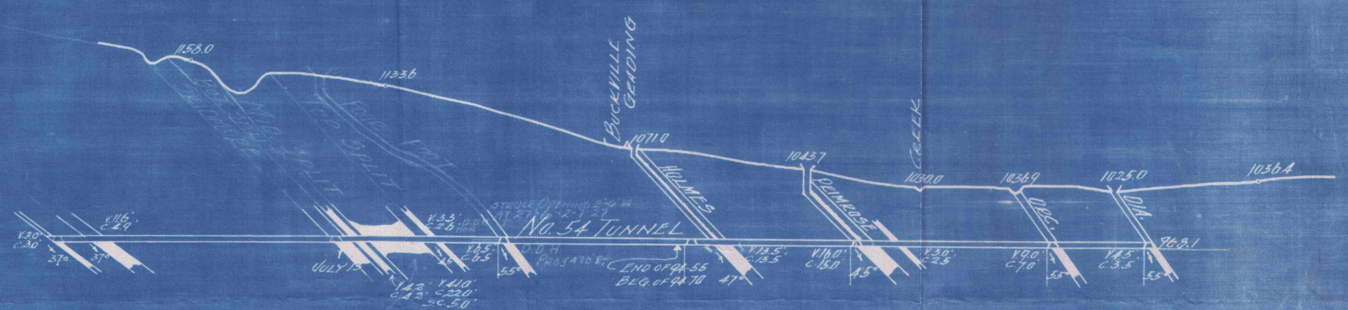
CROSS SECTION THRU No. 54 TUNNEL No. 2 Drift Looking East - Scale: 1"=100'
