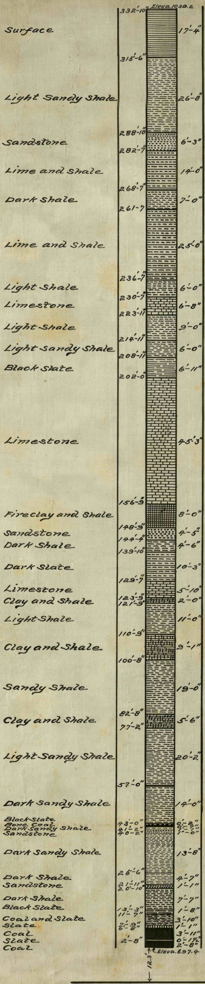
DIAMOND DRILL HOLE No. 2 On Jas White's Farm 1/4 West Rilson Station
