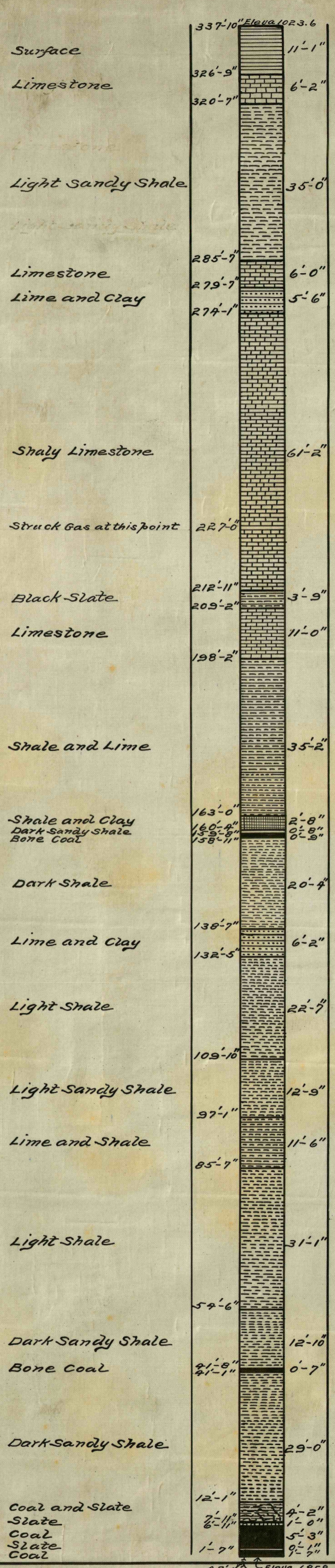
DIAMOND DRILL HOLE No. 3 On Oliver Brown Farm 3/4 mile N.E. Rilson Station
