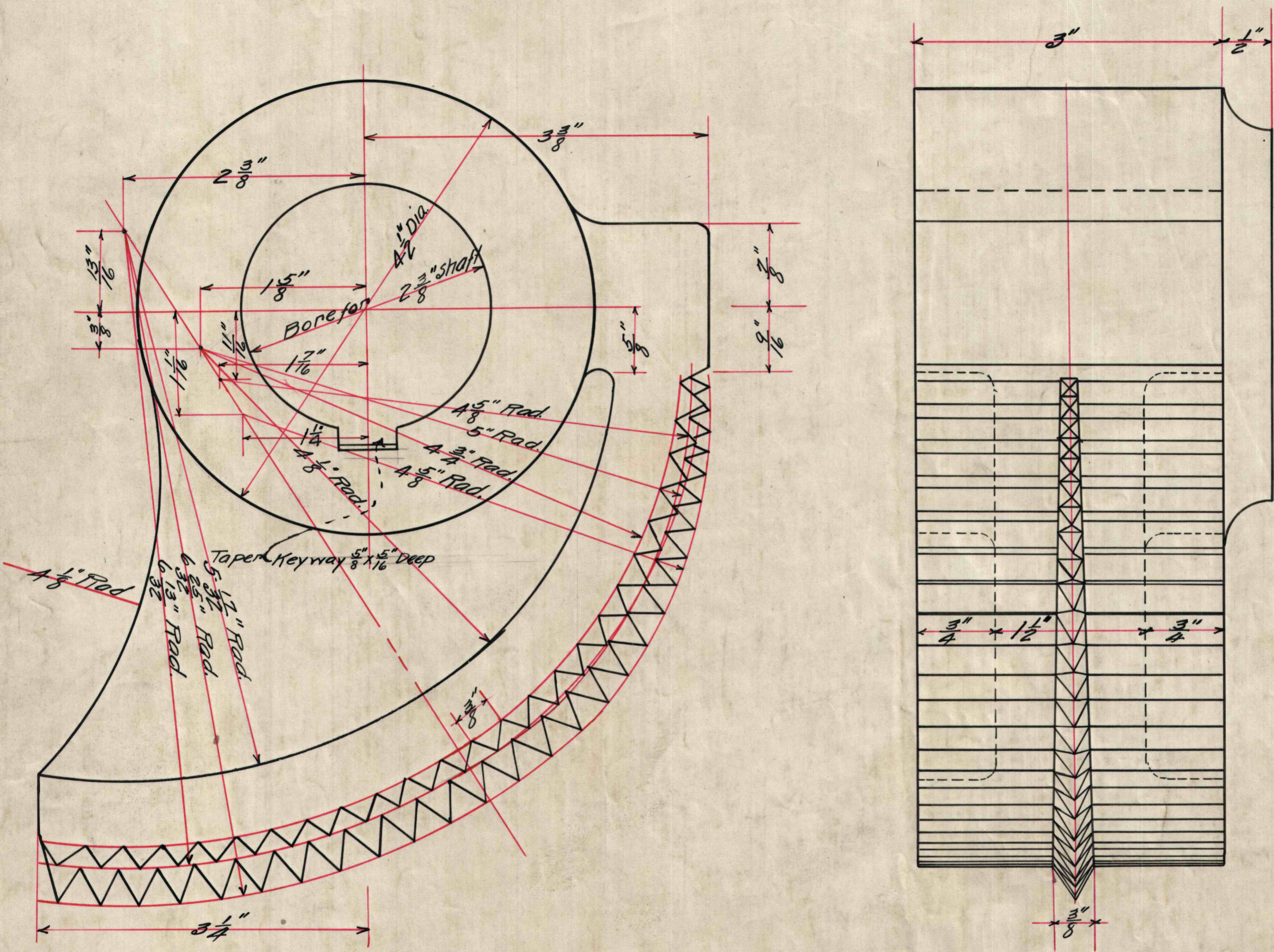
————— Ellsworth Collieries Co. ————— ————— Plan of Safety Catch ————— ————— for Cages at ————— ————— No 3 & 4 Mines ————— ————— Scale - Full Size — Feb. 6 - 1912 ————— Required for one Cage:- 2 - Catches as shown. 2 - " Opp. Hand.
