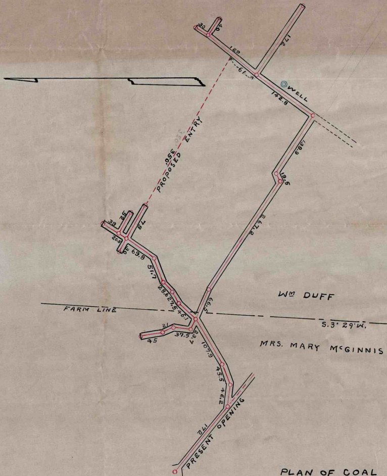
PLAN OF COAL MINE OWNED BY THE UNION COAL & CLAY CO. DARLINGTON TWP. BEAVER CO., PA. SCALE 1" = 100 FT. MAR. 7, 1923 C. O. OBNEY, C. E.
