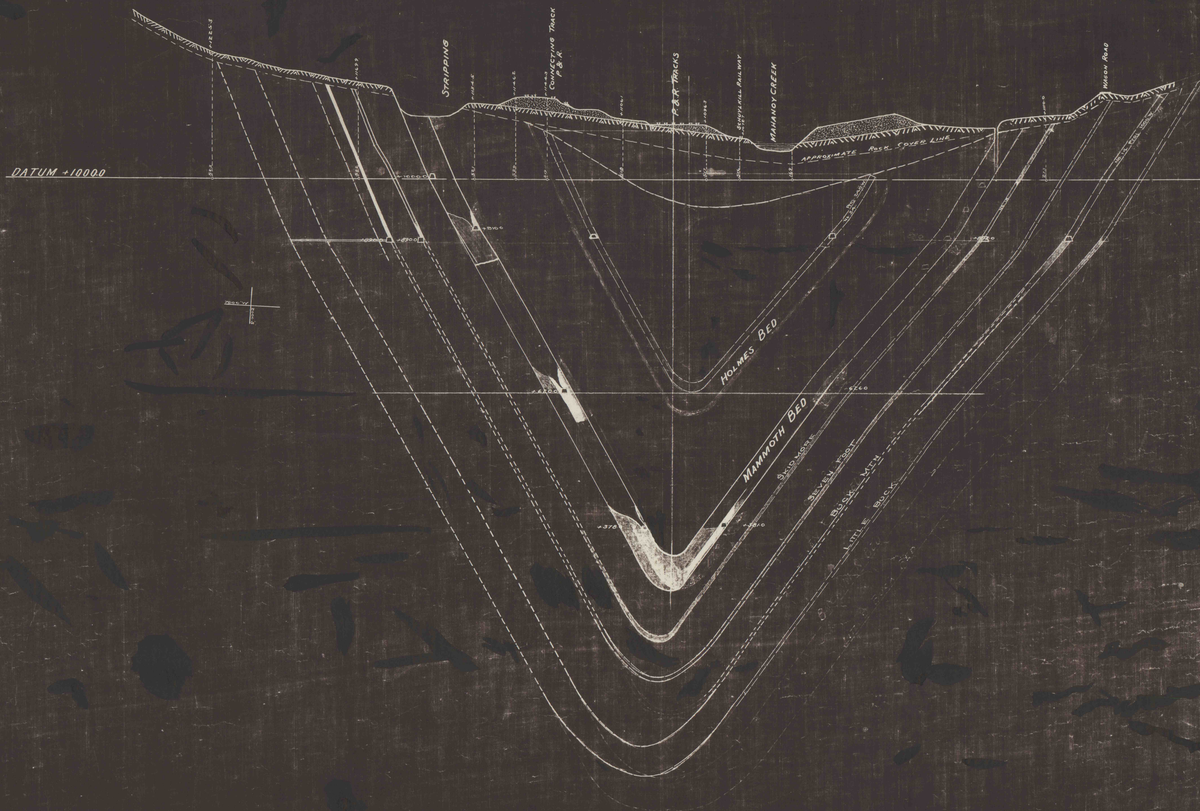
CROSS SECTION THRU BASIN AT WEST BEAR RIDGE COLLIERY 820 FT. EAST OF WEST LINE HARLEIGH BROOKWOOD COAL CO FRACKVILLE PA. SCALE 100 FT. = 1 INCH JULY 1918
