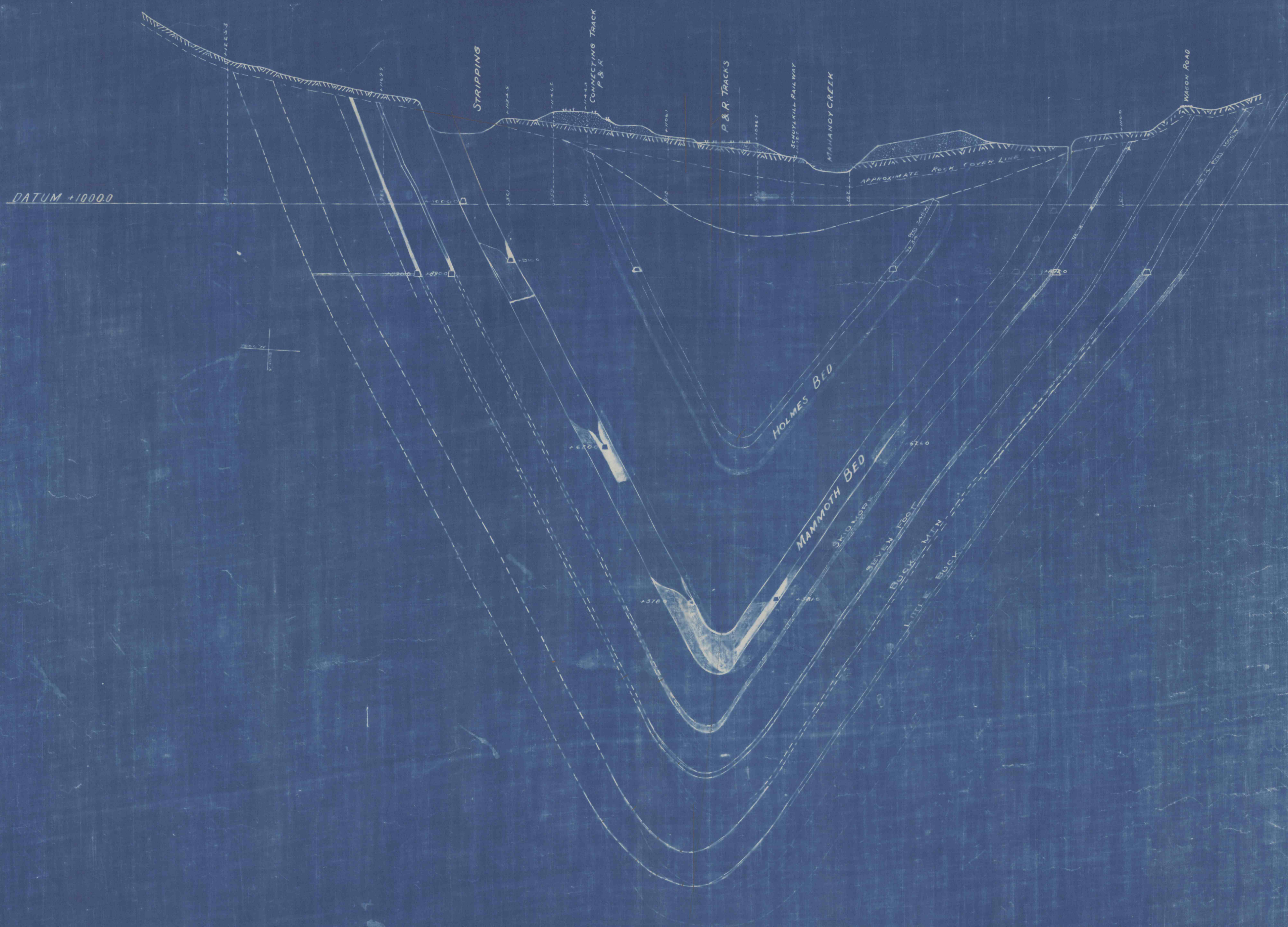
CROSS SECTION THRU BASIN AT WEST BEAR RIDGE COLLIERY 820 FT. EAST OF WEST LINE HARLEIGH BROOKWOOD COAL CO FRACKVILLE PA SCALE 100 FT = 1 INCH JULY 1918
