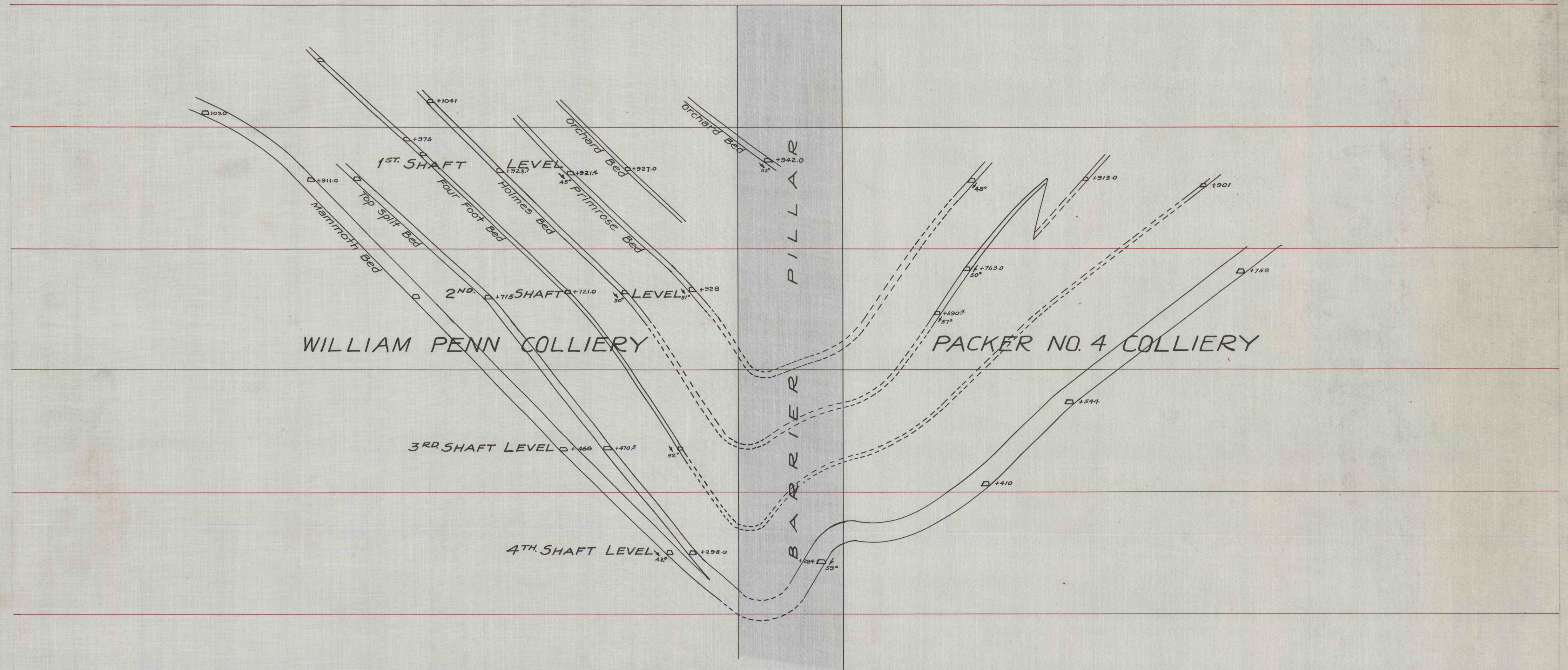
WILLIAM PENN COLLIERY Section 1100 feet West of Shaft Scale 1 inch = 100 feet Pottsville, Pa., James Archbald, April 1917. MINING ENGINEER & AGENT GIRARD ESTATE.
