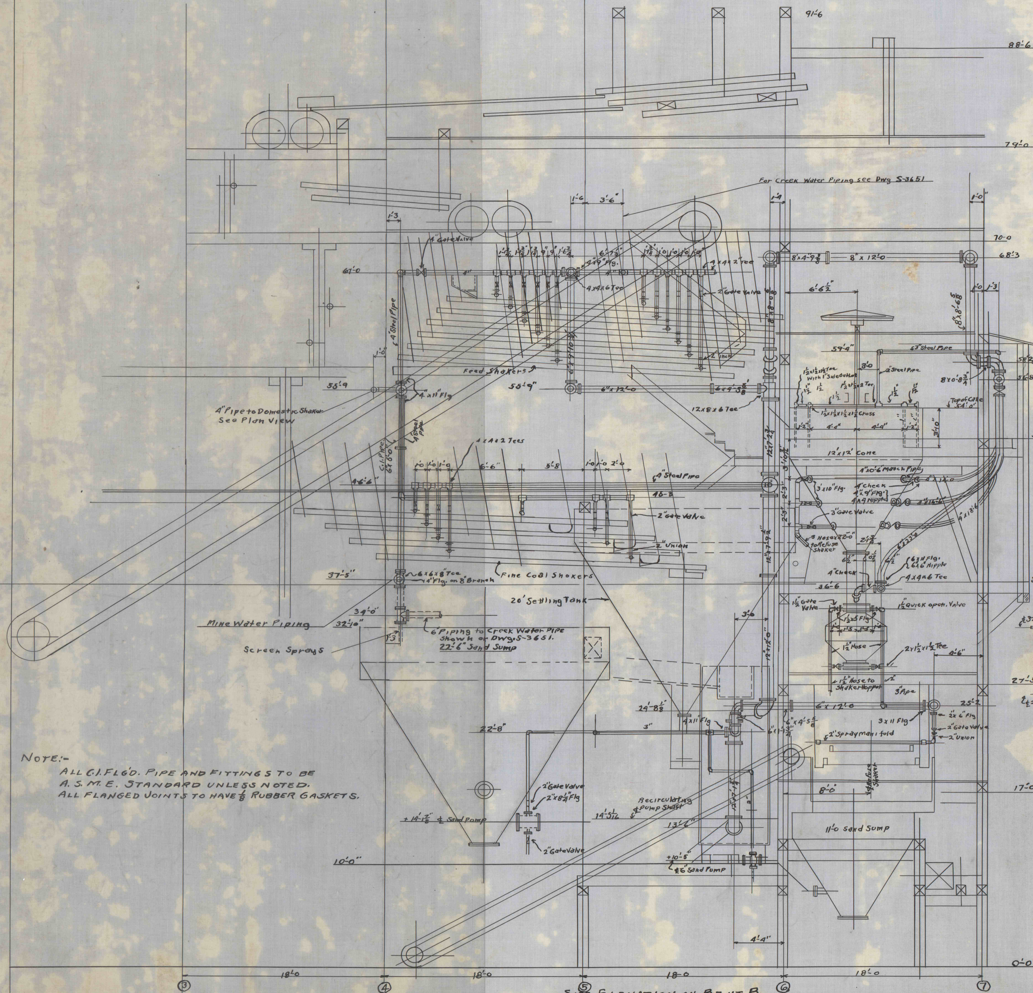
SIDE ELEVATION ON BENT B
