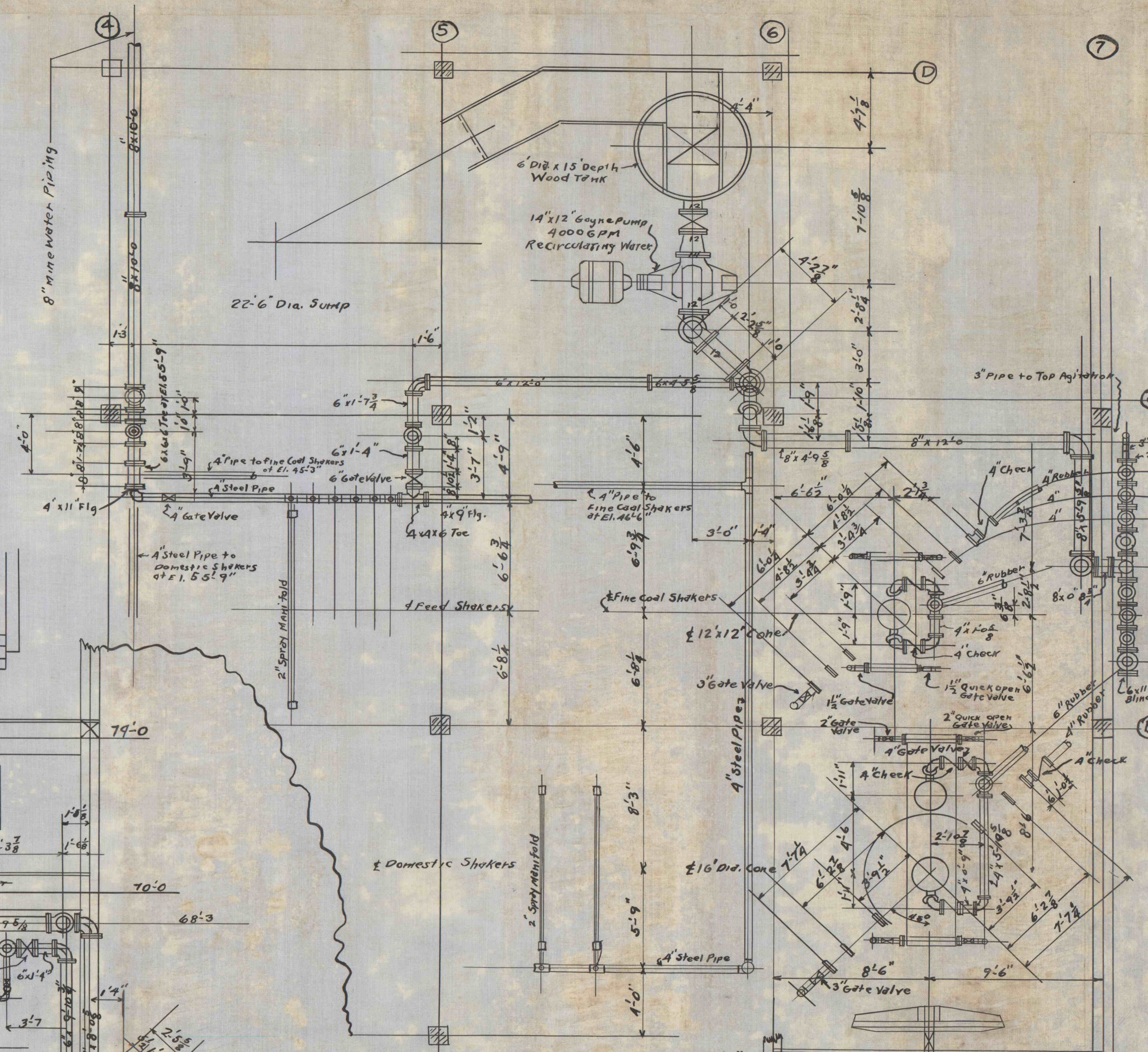
PLAN VIEW OF PIPING
