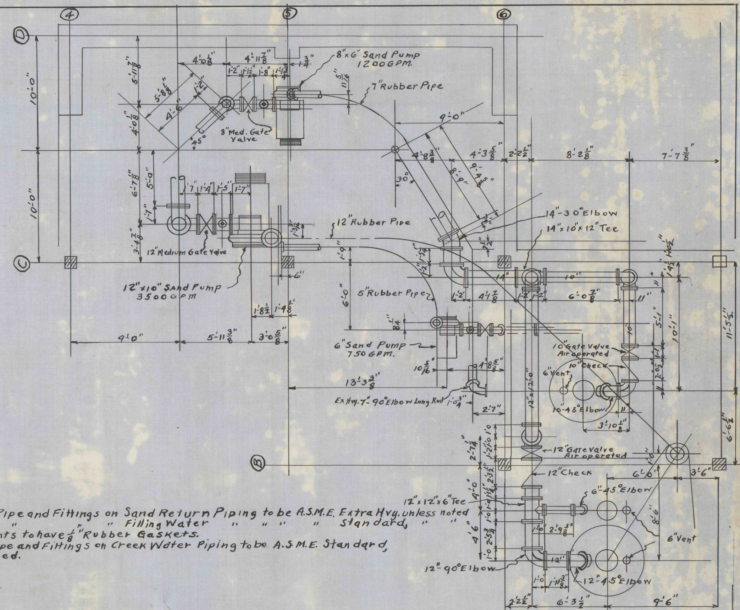
PLAN VIEW OF SAND RETURN PIPING AND FILLING WATER PIPING
