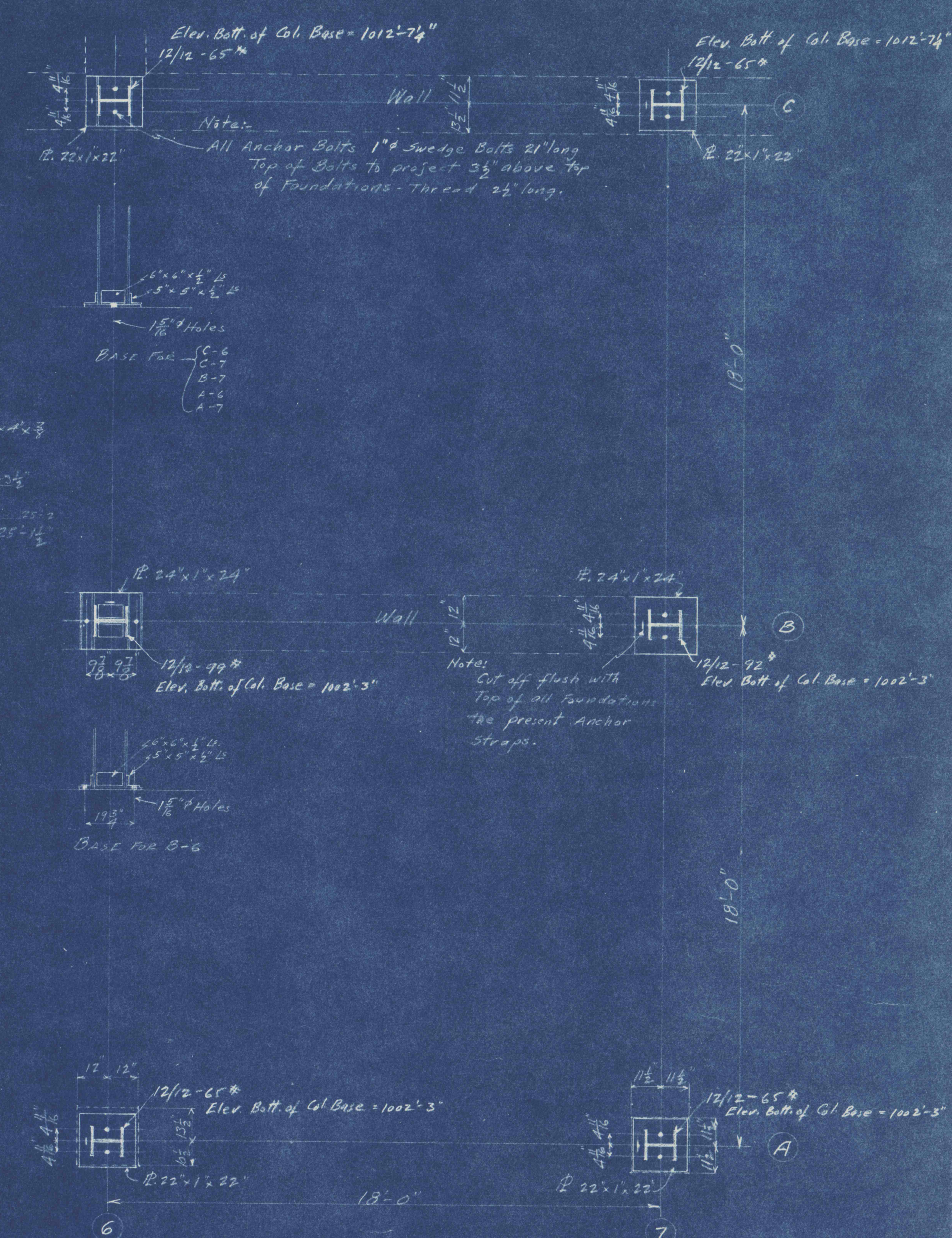
FOUNDATION, COLUMN BASES & ANCHOR BOLT PLAN
