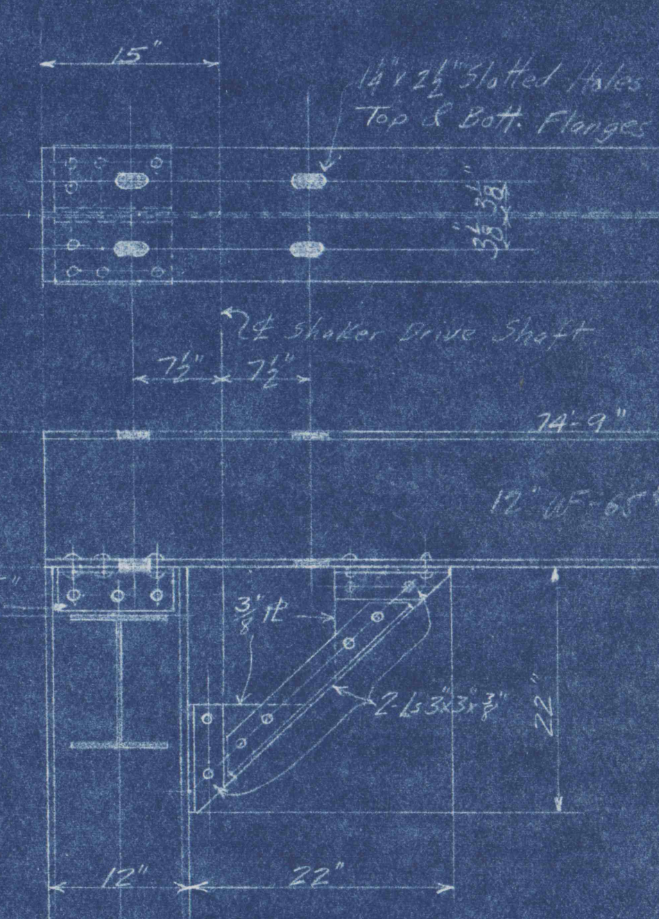
DETAIL SHAKER SHAFT SUPPORT
