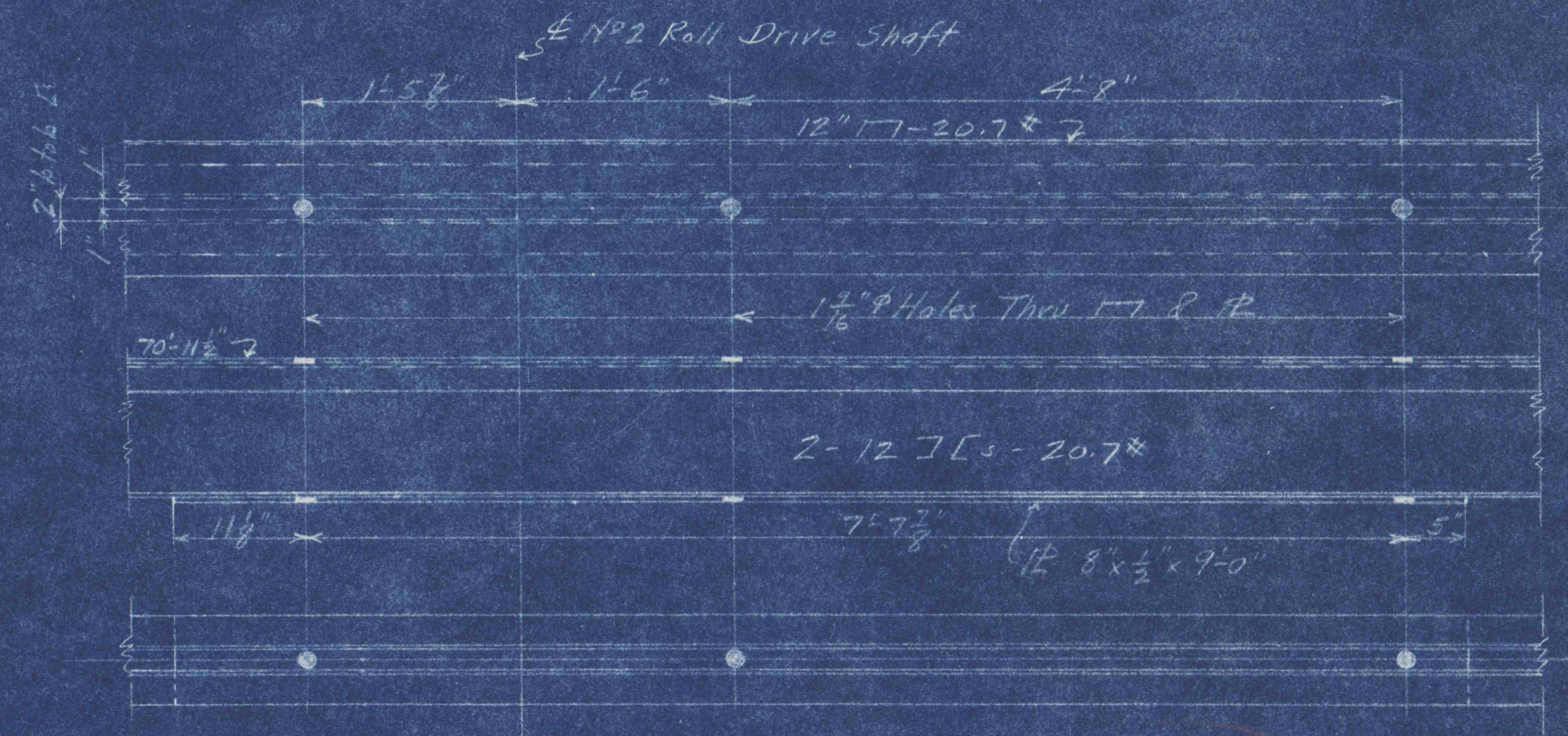
DETAIL NO. 2 ROLL SUPPORT
