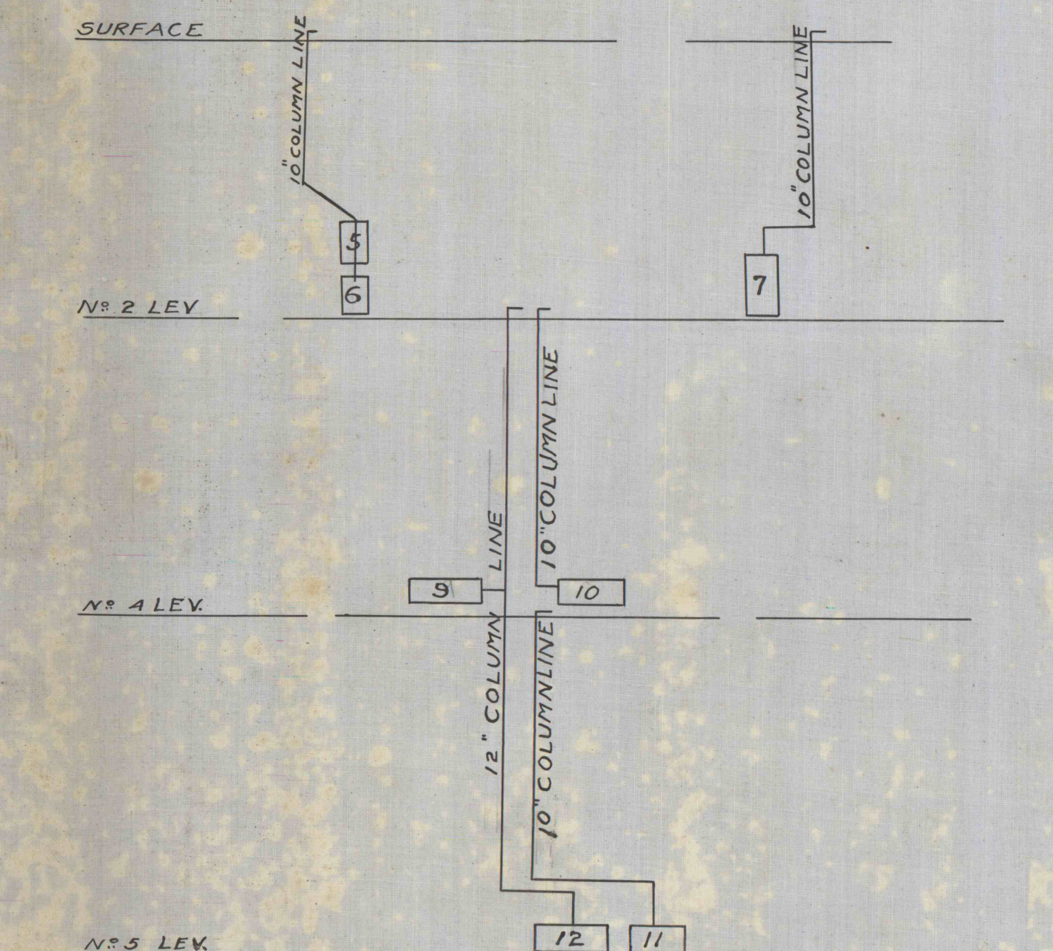
ARRANGEMENT PUMPS AND COLUMN LINES AT PACKER NO. 2 COLLIERY
