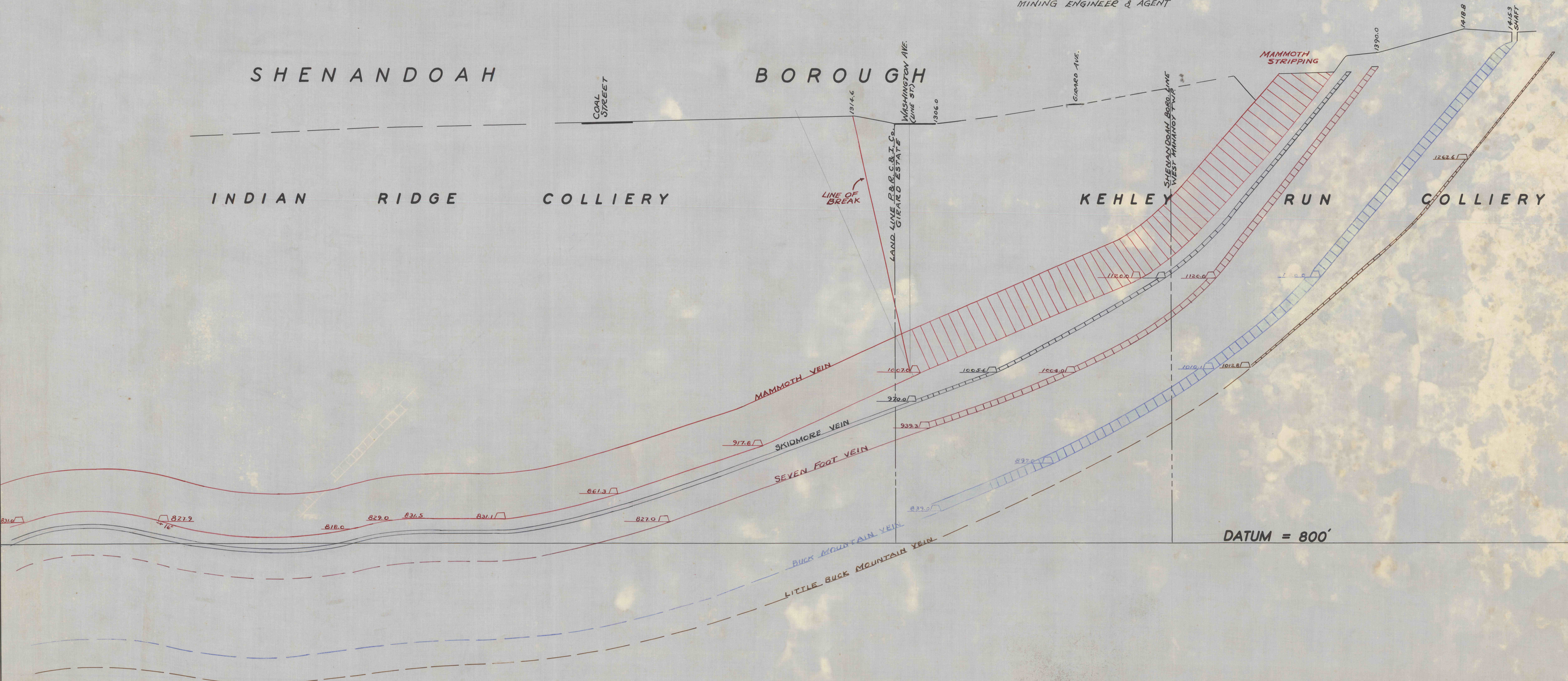
SECTION "H"
