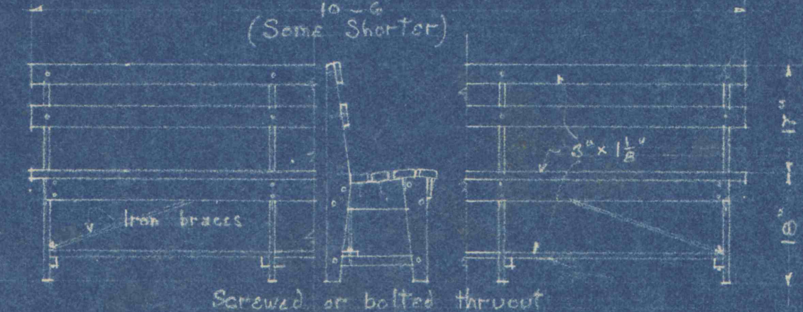
MOVABLE BENCHES for BAND AUDIENCE (1500 ft) May be stacked for storage 1/2" Scale
