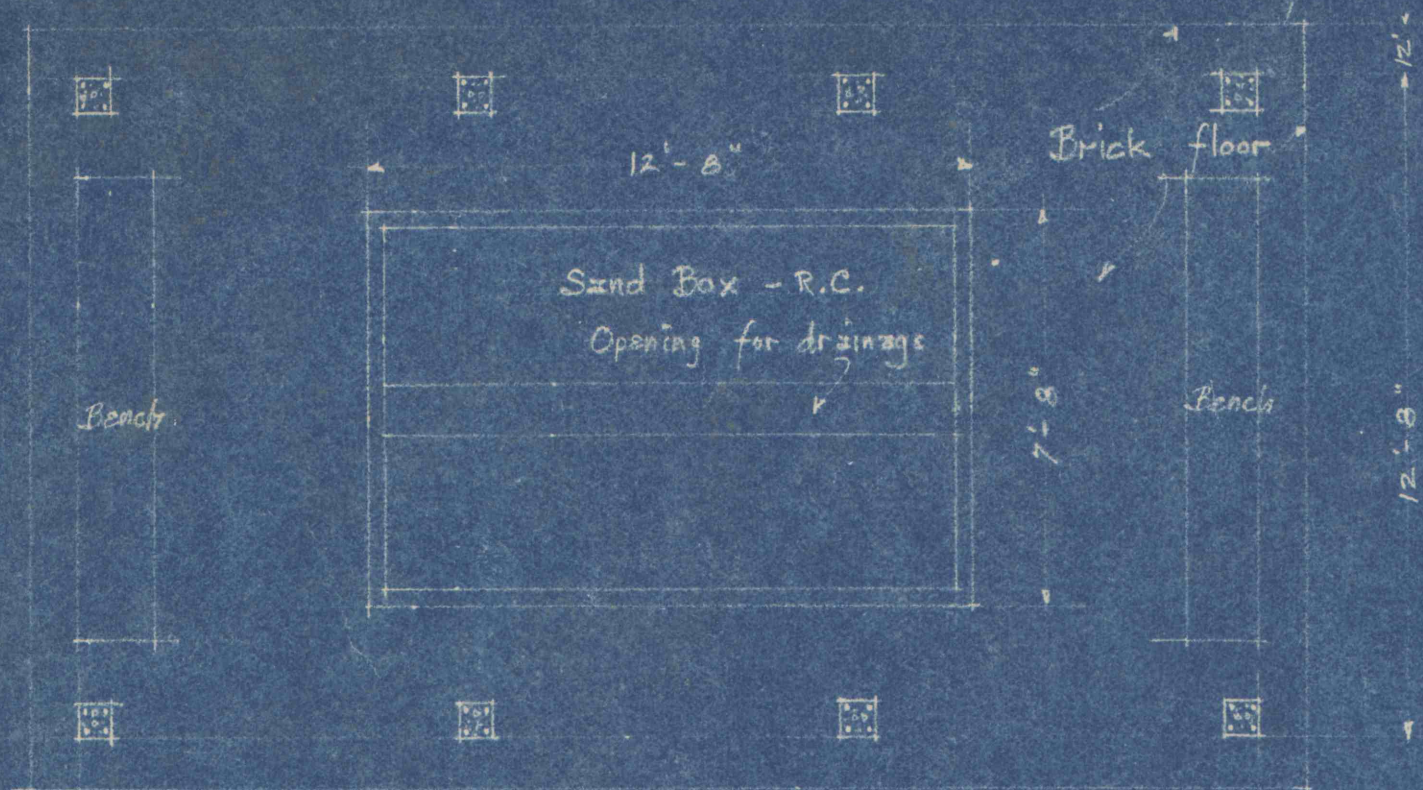
SAND BOX AND SHELTER ① 1/4" Scale
