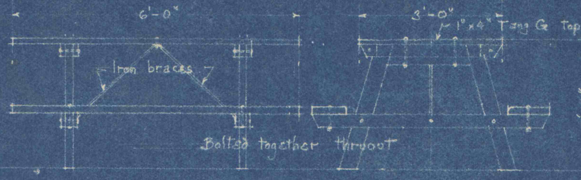
LUNCH TABLE ⑤ Demountable for winter storage. 1/2" Scale
