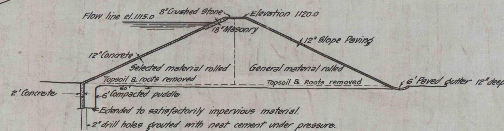
TYPICAL SECTION OF EMBANKMENT
