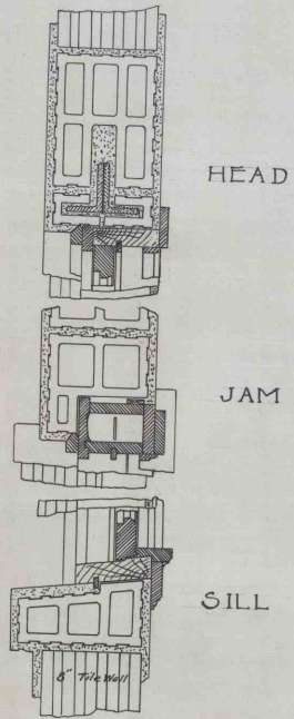
DETAIL SECTION OF WINDOW
