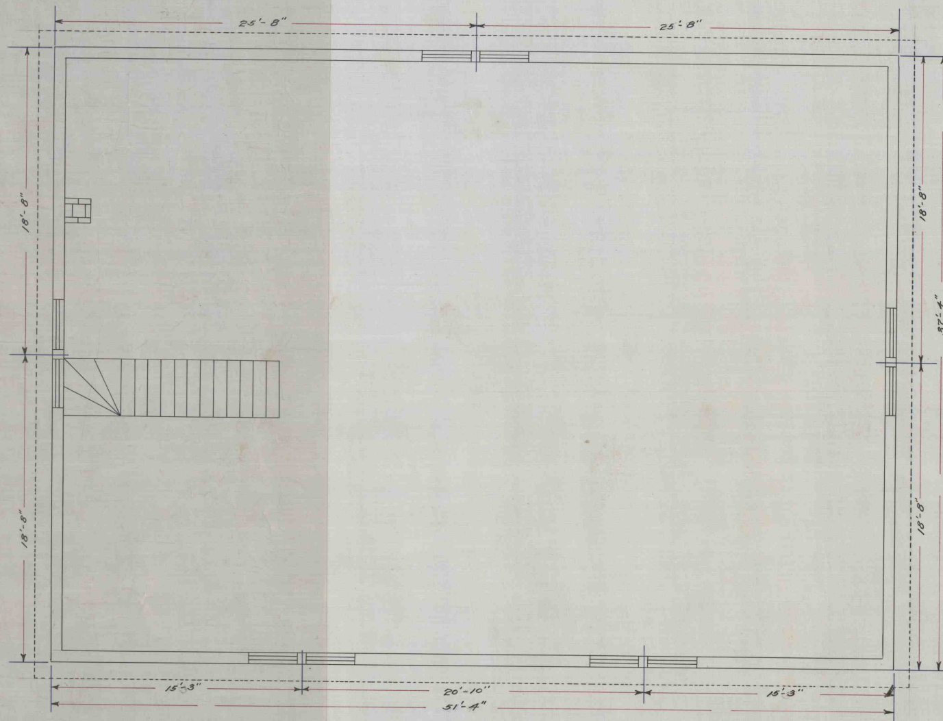
~ Second Floor Plan ~ ~ Scale 1/4" = 1 ft ~
