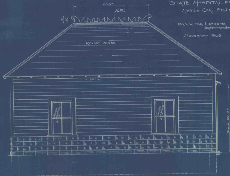
SIDE ELEVATION. Scale: 4 Feet per inch.
