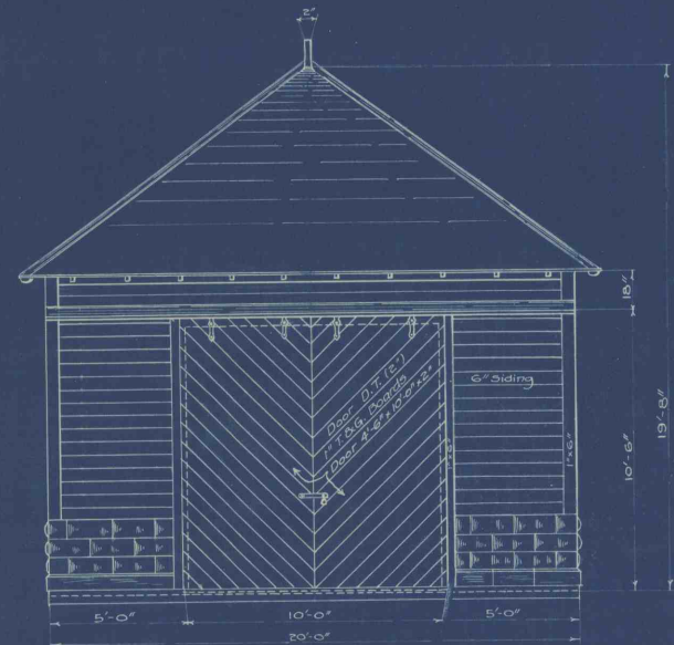
FRONT ELEVATION. Scale: 4 Feet per inch.
