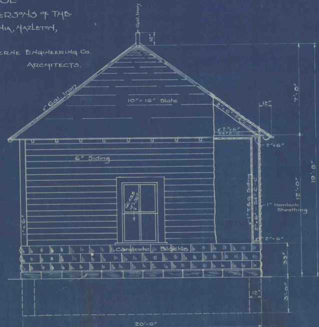
REAR ELEVATION. Scale: 4 Feet per inch.
