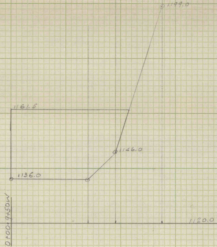
SECTION 1+86
