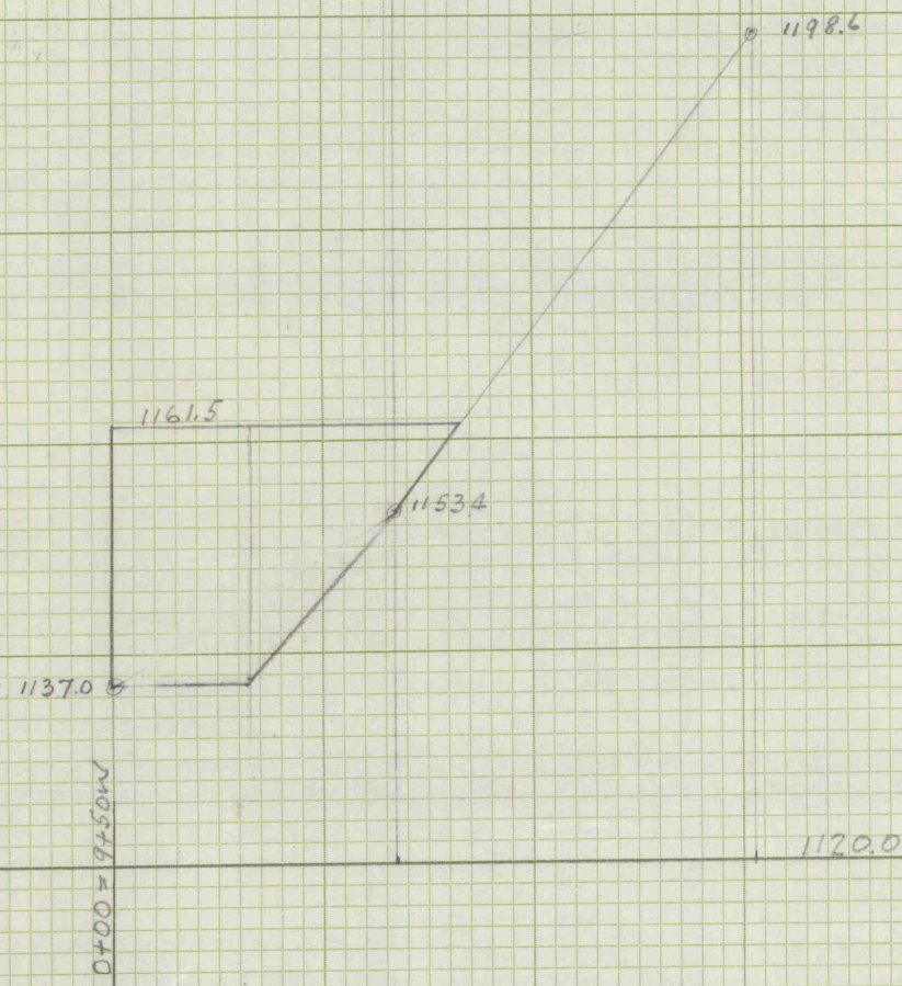
SECTION 1+50 S
