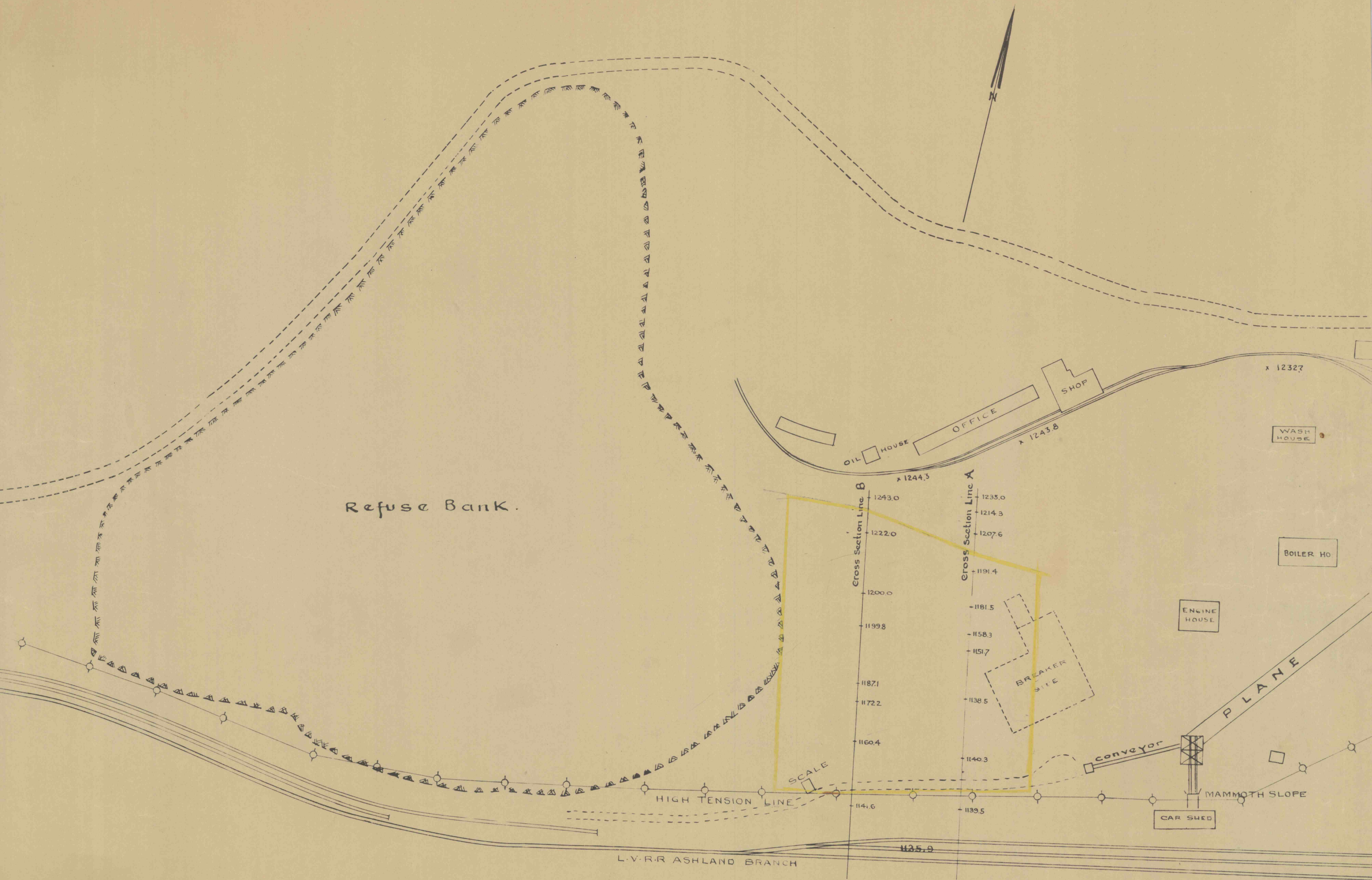
Packer No. 4 Colly. Plan showing Proposed Mammoth Vn. Stripping Scale 100' = 1" Dec. 11, 1939 Eng. Dept Locust Coal Co.
