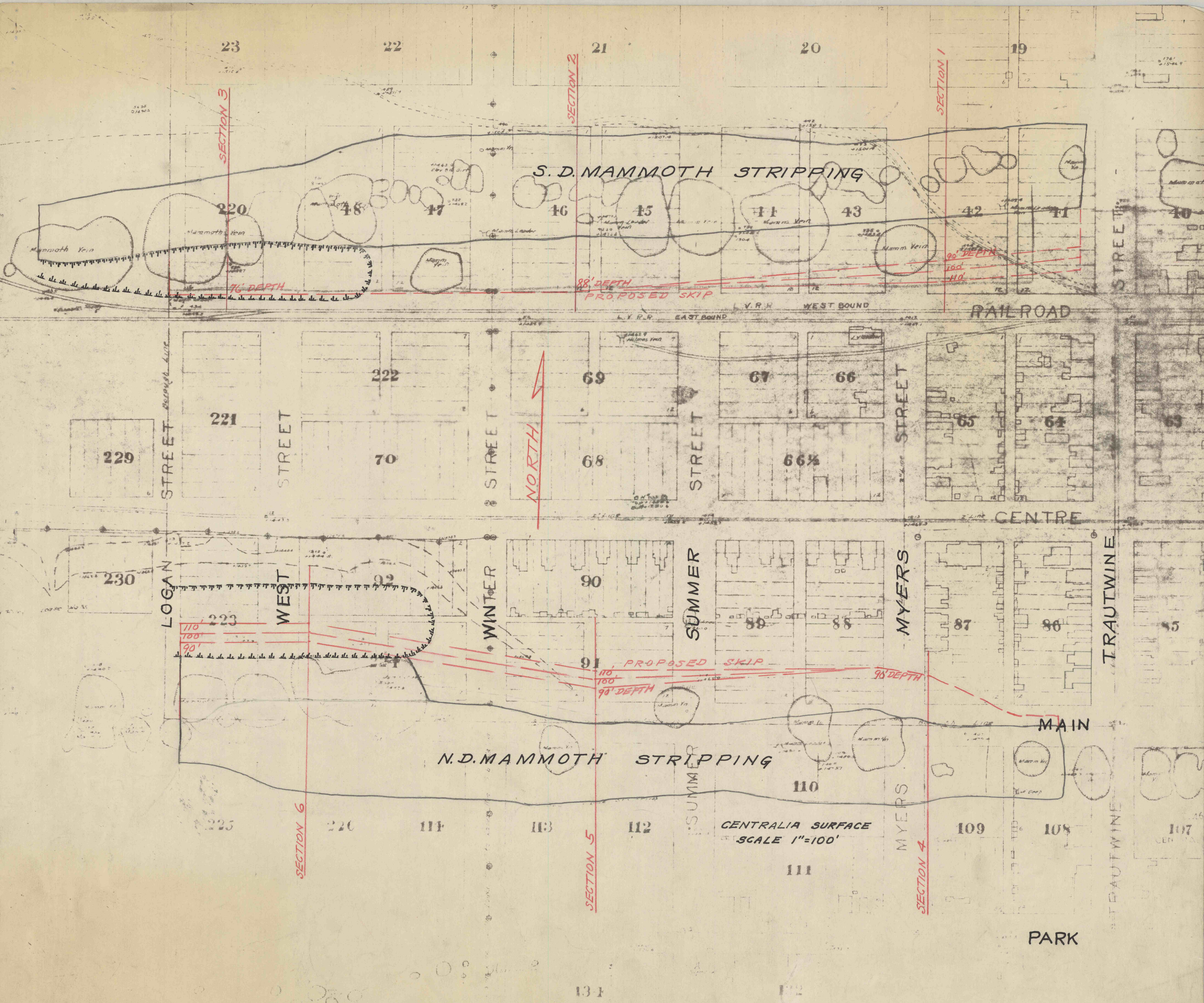
PROPOSED N&S.D. MAMMOTH STIPPINGS AT CENTRALIA SCALE — PLAN 1"=100' SECTIONS 1"=20'. Nov. 1, 1951
